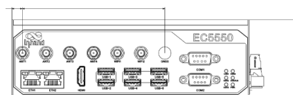
Interface Diagram
