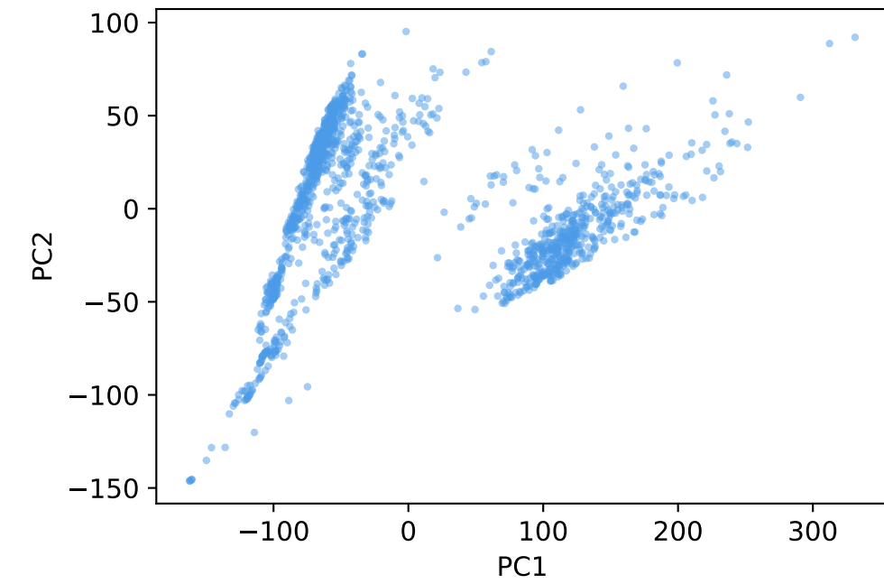
6. PCA final (SVD) PC1=42.0% PC2=7.1%
