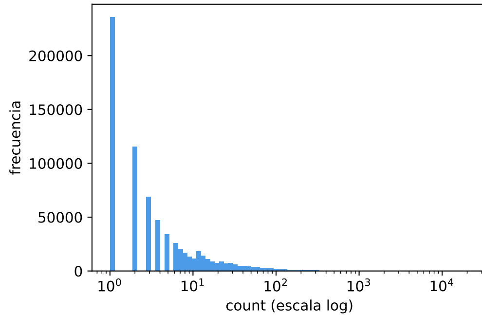
1. Conteos crudos (raw counts, ceros excluidos de la vista log) skew=133.17 mean=5.02 sd=74.39
