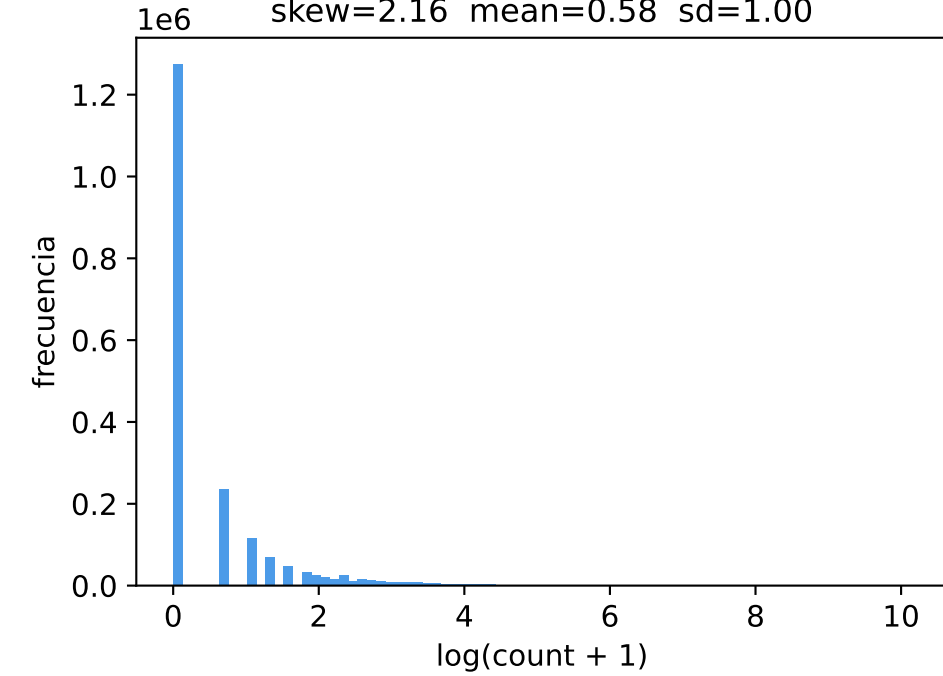
3. Tras pseudo-count (+1) y log skew=2.16 mean=0.58 sd=1.00
