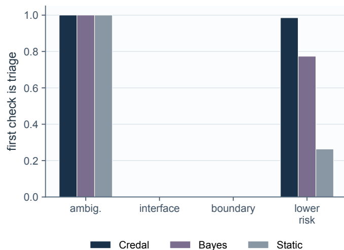
D The worst explanation changes with history
