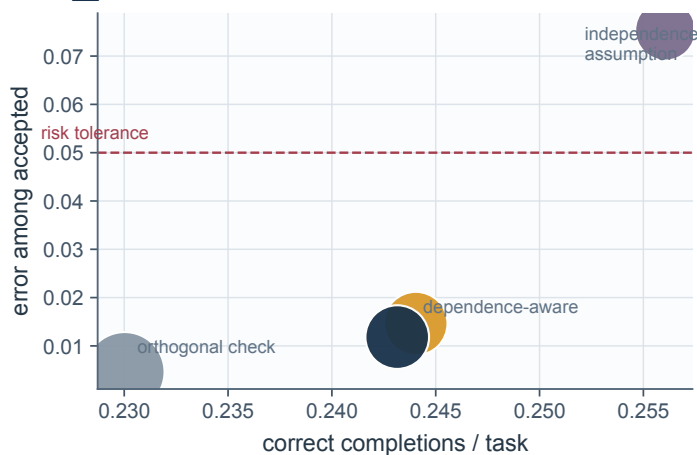
A Dependence controls false confidence
