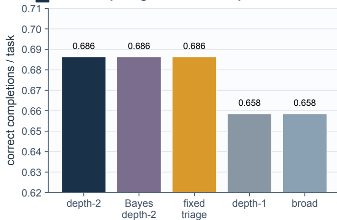
B Two-step triage recovers completions
