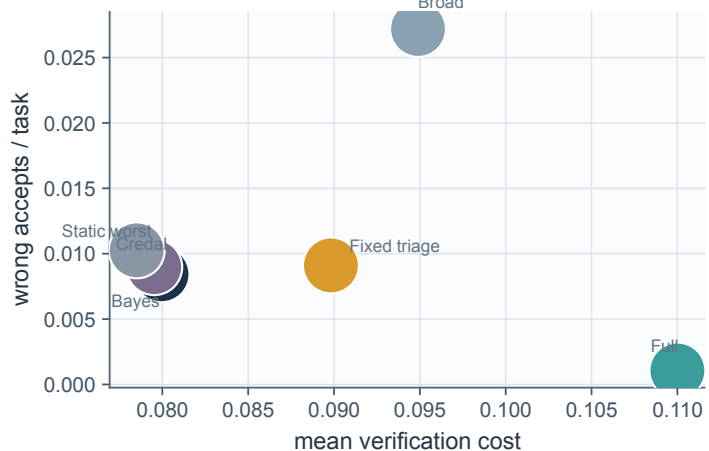
C Active selection improves the cost--risk frontier
