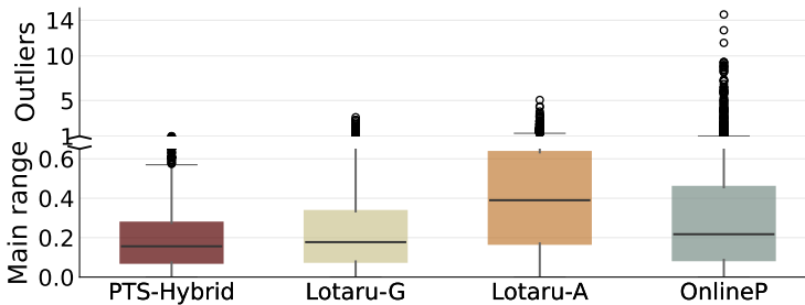
Fig. 8. Box plot of per-task relative prediction errors. Lower panel (0–0.6) shows the main range and whiskers; upper panel (1–14) shows outliers. PTS-Hybrid's outliers stay below 2x, while OnlineP's reach 14x.
