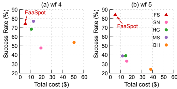
Figure 10: Total cost vs. success rate for wf-4 and wf-5. The top-left region indicates higher success at lower cost. On wf-4, FaaSpt (red triangle) has the lowest cost while MScheduler reaches slightly higher success at over twice the cost. On wf-5, FaaSpt leads on both axes with all four baselines clustering at higher cost and lower success.
