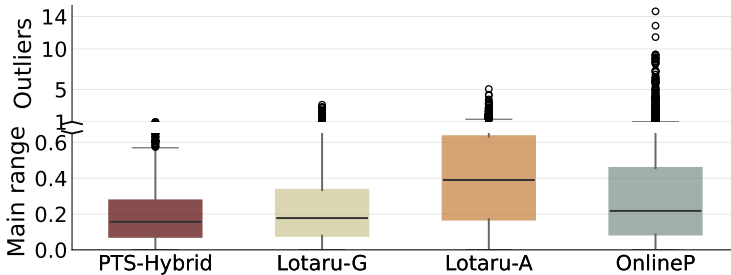
Fig. 8. Box plot of per-task relative prediction errors. Lower panel (0–0.6) shows the main range and whiskers; upper panel (1–14) shows outliers. PTS-Hybrid’s outliers stay below 2\times , while OnlineP’s reach 14\times .
