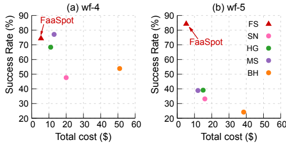
Figure 10: Total cost vs. success rate for wf-4 and wf-5. The top-left region indicates higher success at lower cost. On wf-4, FaaS (red triangle) achieves the lowest total cost while MS achieves slightly higher success at more than twice the cost. On wf-5, FaaS leads on both axes with all four baselines clustering at higher cost and lower success.
