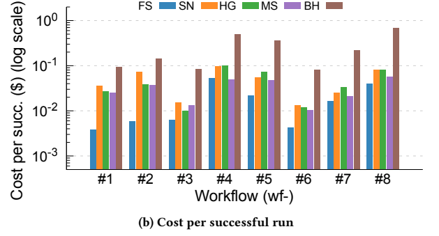
Figure 9: Success rate and cost per success for each workflow and baseline. (a) Success rate across eight workflows: FaaS achieves the highest success rate on seven of eight workflows, with the largest margin on wf-5 (+43 pp over the nearest baseline). (b) Cost per successful run (log scale, lower is better): FaaS achieves the lowest cost per success on seven of eight workflows. ‘FS’: FaaS, ‘SN’: Snape, ‘HG’: Hourglass, ‘MS’: MScheduler, and ‘BH’: Burst-HADS.
