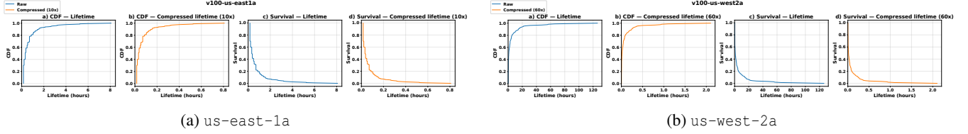
Figure 10: Lifetime and survival distributions for V100 spot instances, derived from availability traces in [56]. Panels (a) and (b) in each subfigure show the CDF of instance lifetime in raw and time-compressed form; panels (c) and (d) show the corresponding Kaplan-Meier survival curve. The time compression factor ( 10\times for us-east-1a, 60\times for us-west-2a) is a configurable parameter of the Spot Emulator, set independently per region to fit evaluation run-time constraints; it is not derived from the trace data itself. The Spot Emulator samples instance lifetimes from these distributions to replay preemption events during evaluation.
