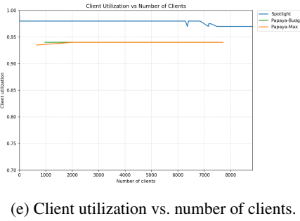
Figure 15: FedYogi results: client utilization, queue time, and cost under the single-wave trace.
