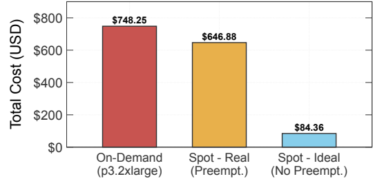
Figure 2: Aggregator cost to train ResNet-18 on CIFAR-100 to convergence on a p3.2xlarge instance (1,198 rounds [49]). Without fault tolerance, preemptions force full restarts, raising the spot cost from an ideal $84.36 to $646.88, close to the on-demand cost of $748.25.
