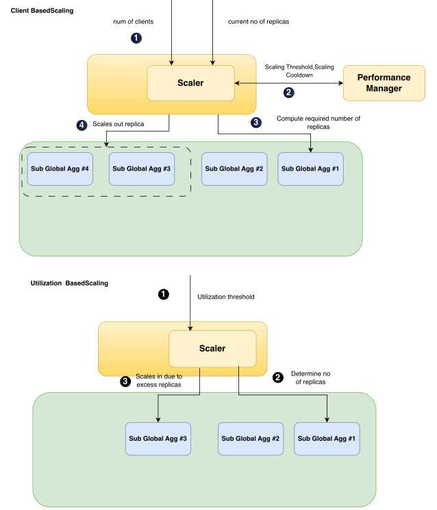
Figure 7: Scaling Algorithm
