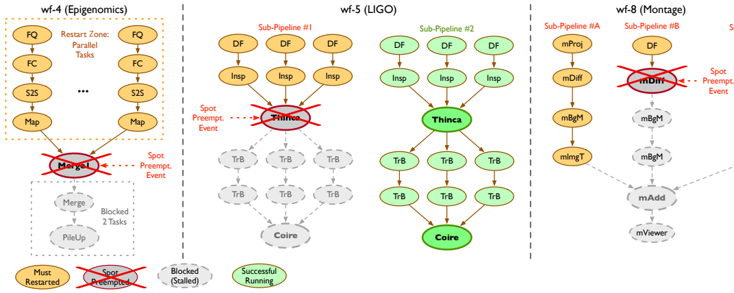
Figure 3: Three representative DAG workflows and the cascade failures at their synchronization barriers. wf-4 (Epigenomics [5]), wf-5 (LIGO [5]), and wf-8 (Montage [5]) each contain fan-out nodes and synchronization barriers. Under naive deployment, a preemption of any parallel task feeding a barrier fails the entire run: the preempted task (red), every other branch that must restart with it (orange), and the downstream tasks left stalled at the barrier (gray). For wf-5, the two sub-pipelines contrast a preemption-hit branch with an unaffected one.
