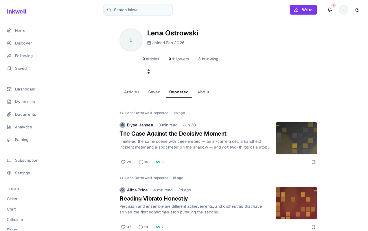
Figure 7.11 – The Reposted tab of a profile
