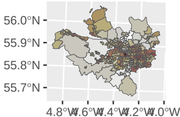
sd risk
