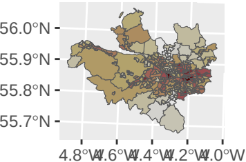
mean risk
