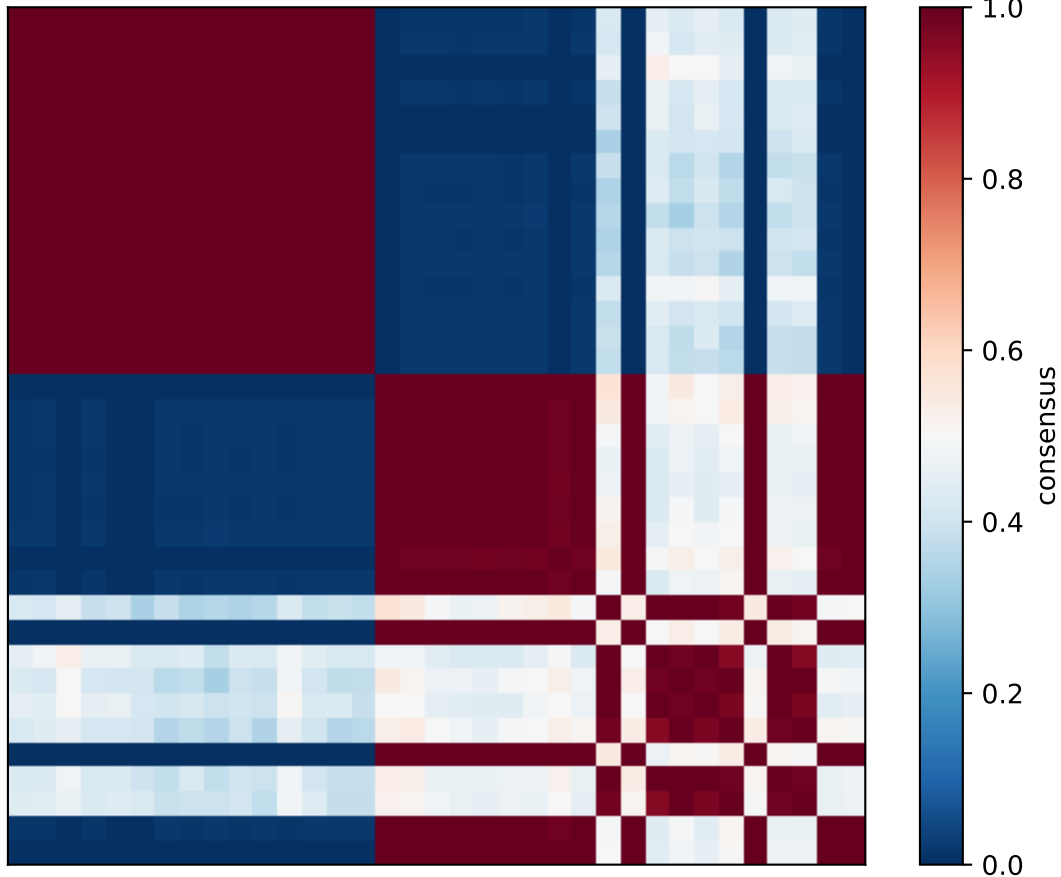
Consensus NMF k=2
