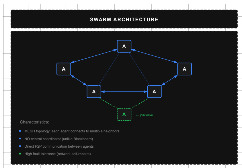
Figure 7: Swarm architecture with emergent coordination
