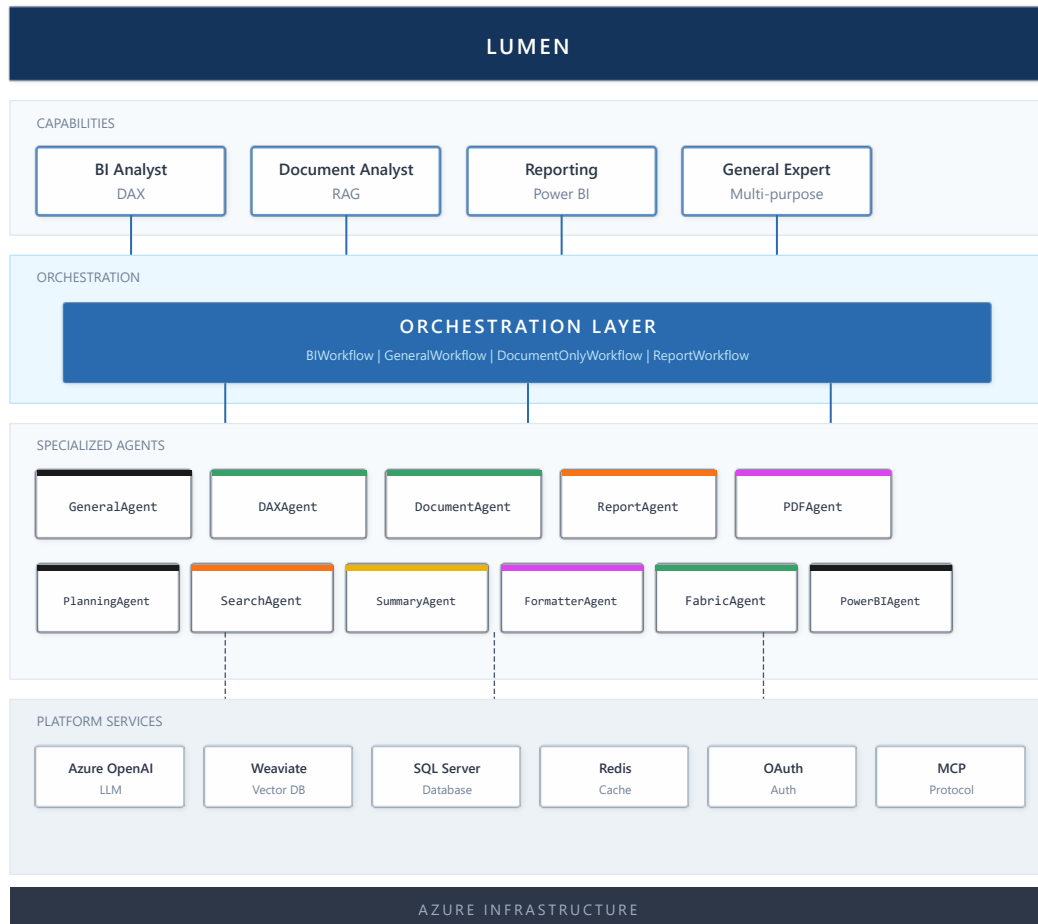
Figure 10: Complete LUMEN architecture showing all layers and components
