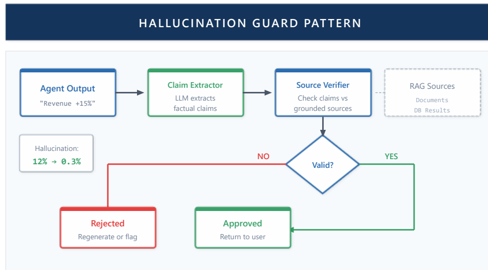
Figure 18: HallucinationGuard Pattern: validates agent outputs against grounded sources, reducing hallucinations from 12% to 0.3%
