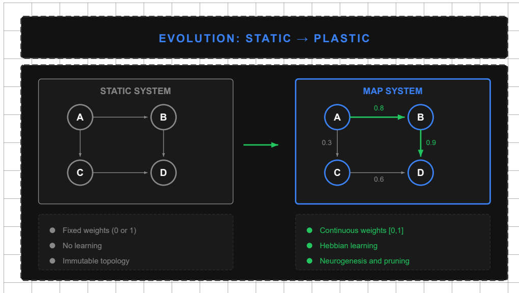
Figure 21: Evolution from static to plastic systems in MAP
