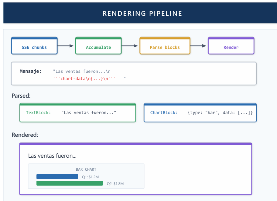
Figure 17: Visualization rendering pipeline
