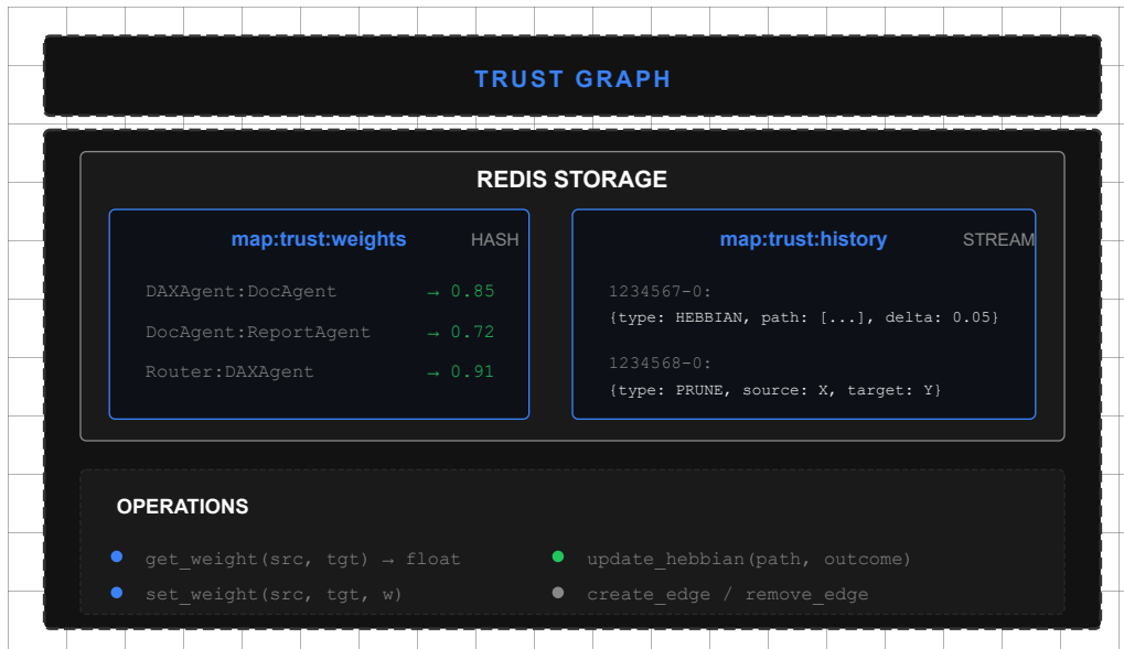
Figure 22: Trust graph structure in MAP
