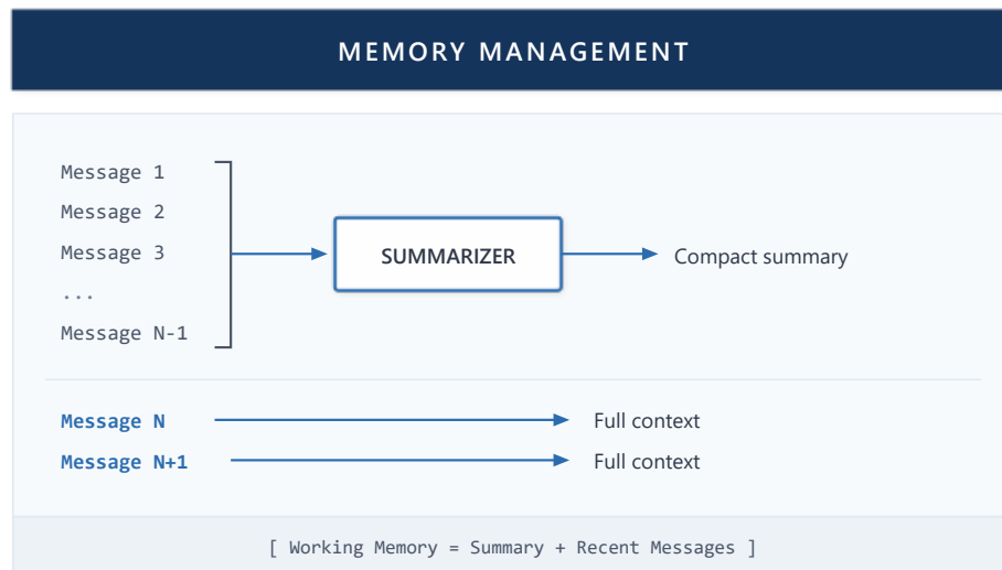
Figure 11: Multi-tier memory architecture
