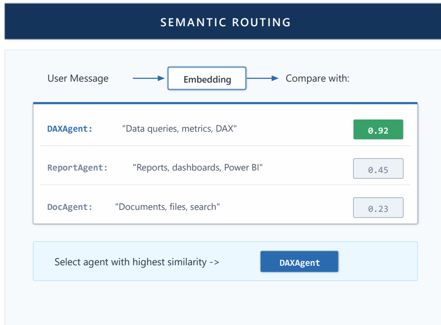
Figure 12: Two-layer routing: keywords first, then semantic
