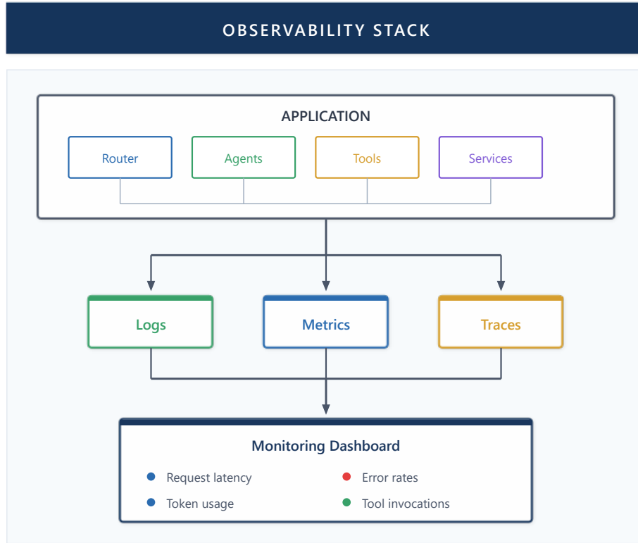
Figure 20: Complete observability stack
