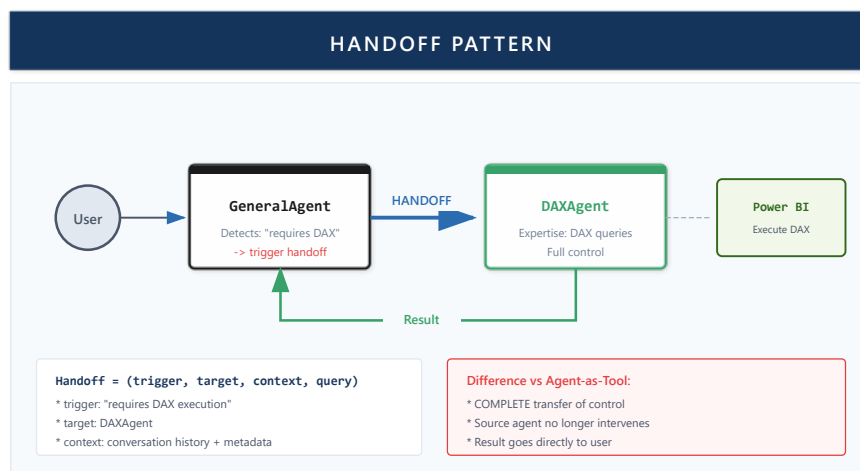
Figure 15: Handoff Pattern—Complete Transfer of Control
