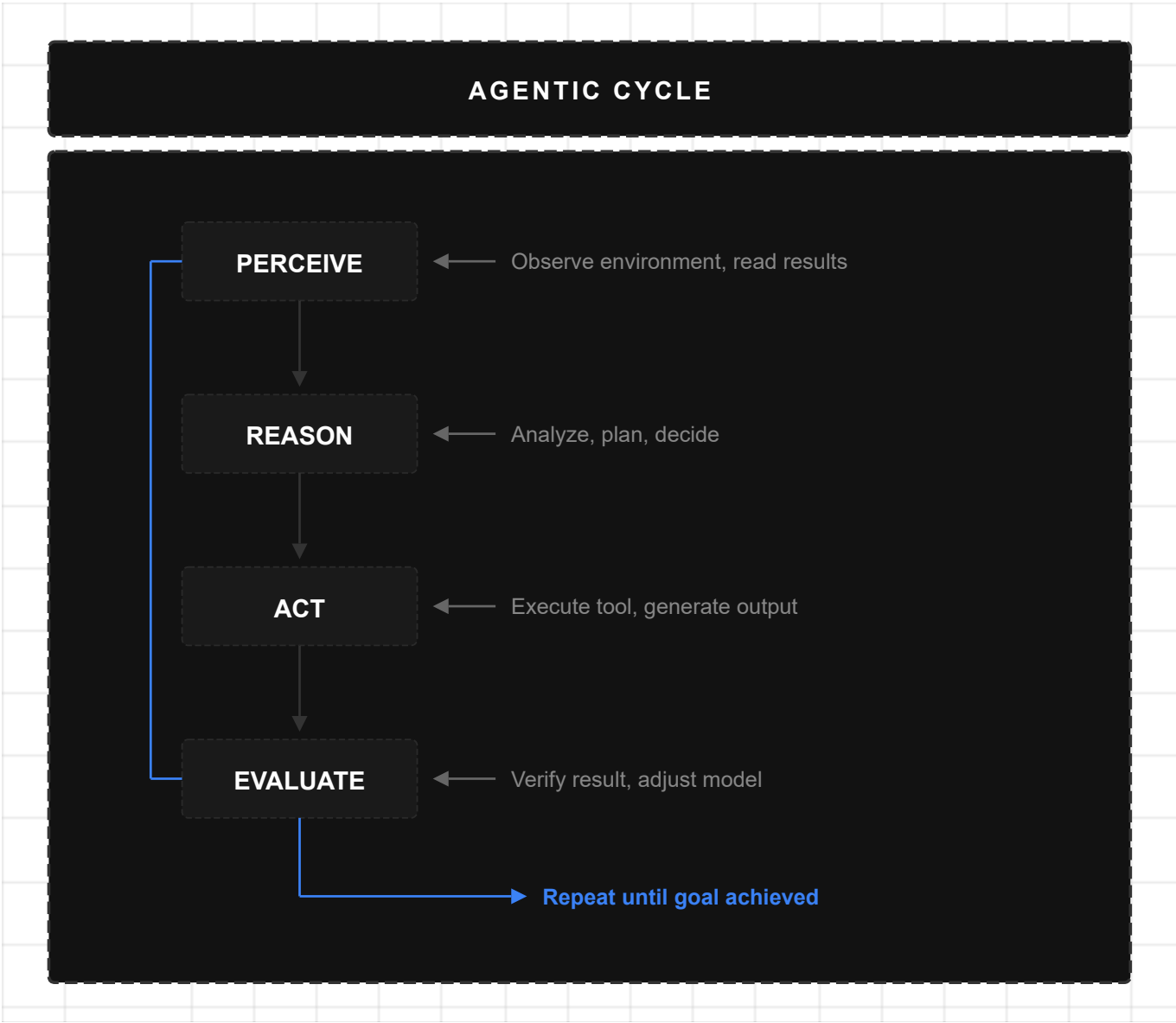
Figure 3: Agentic Cycle
