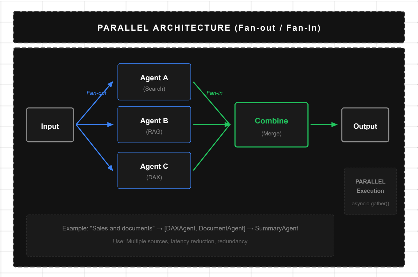
Figure 15: Parallel Architecture
