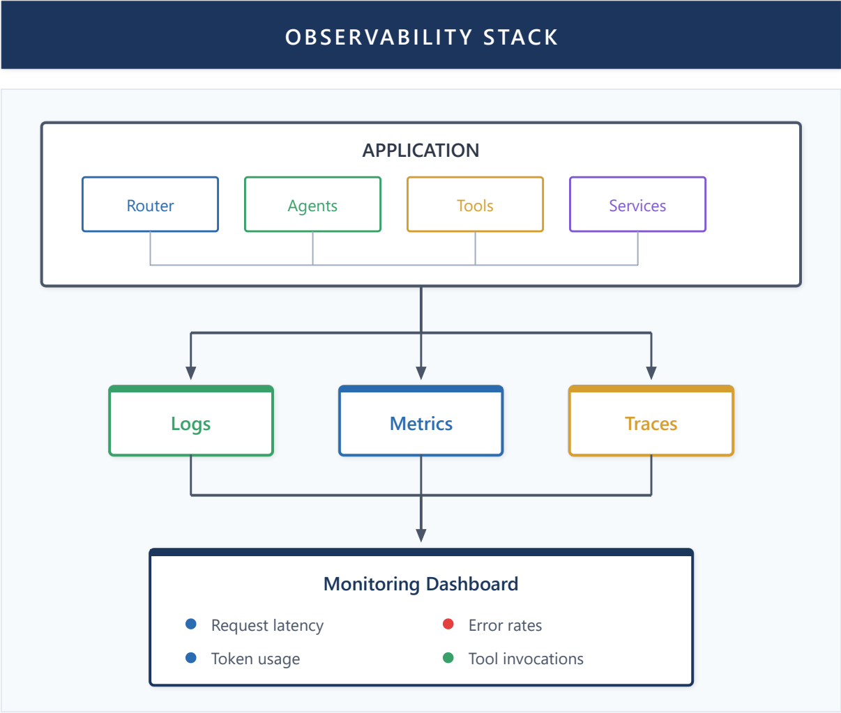
Figure 36: Observability Stack
