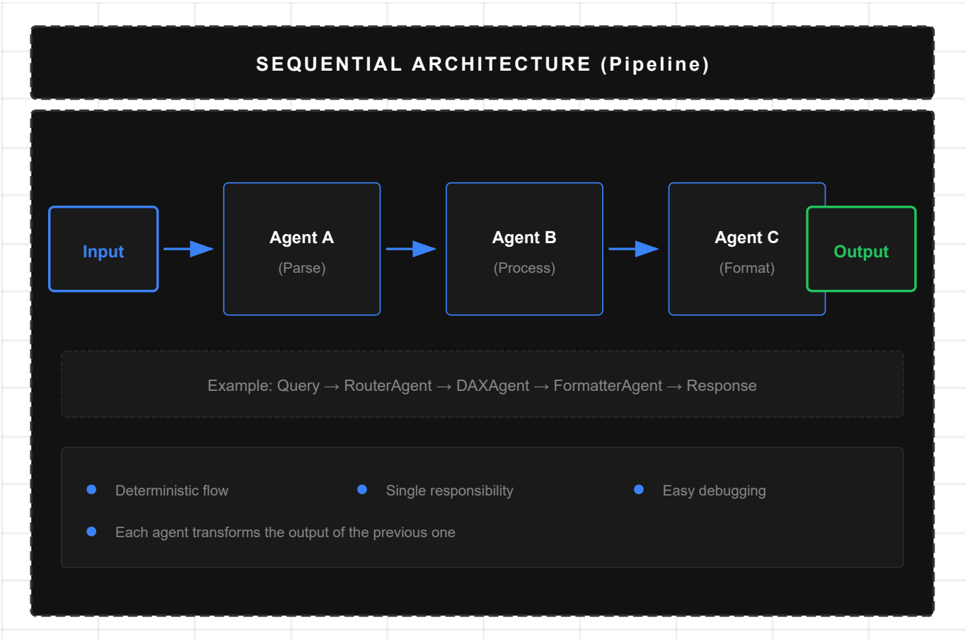
Figure 14: Sequential Architecture
