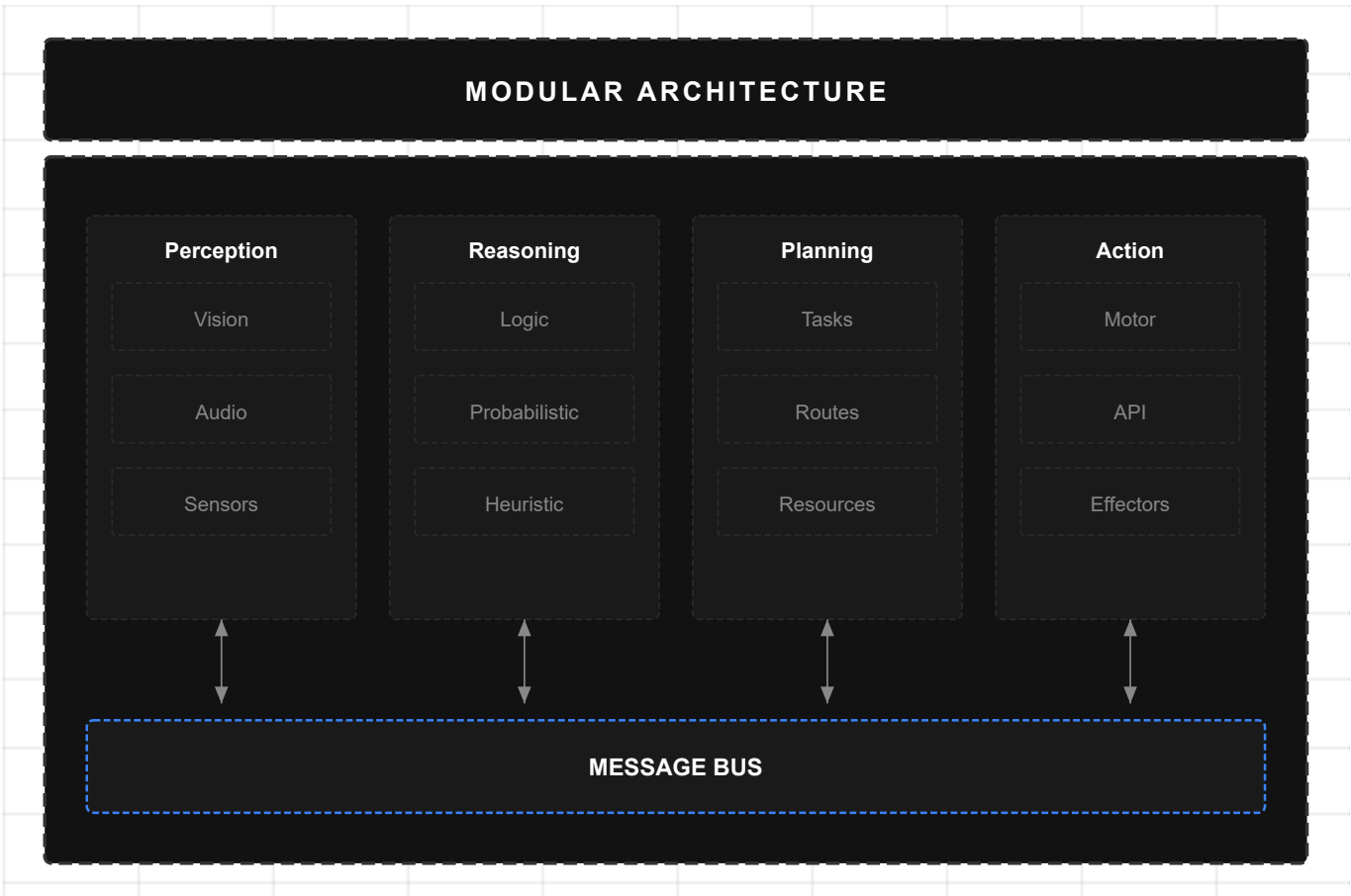
Figure 9: Modular Architecture
