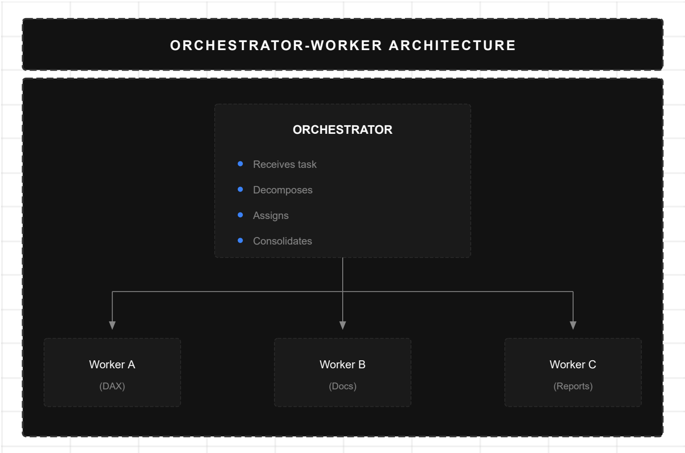
Figure 11: Orchestrator-Worker Architecture
