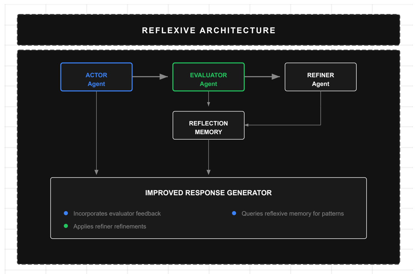
Figure 16: Reflexive Architecture
