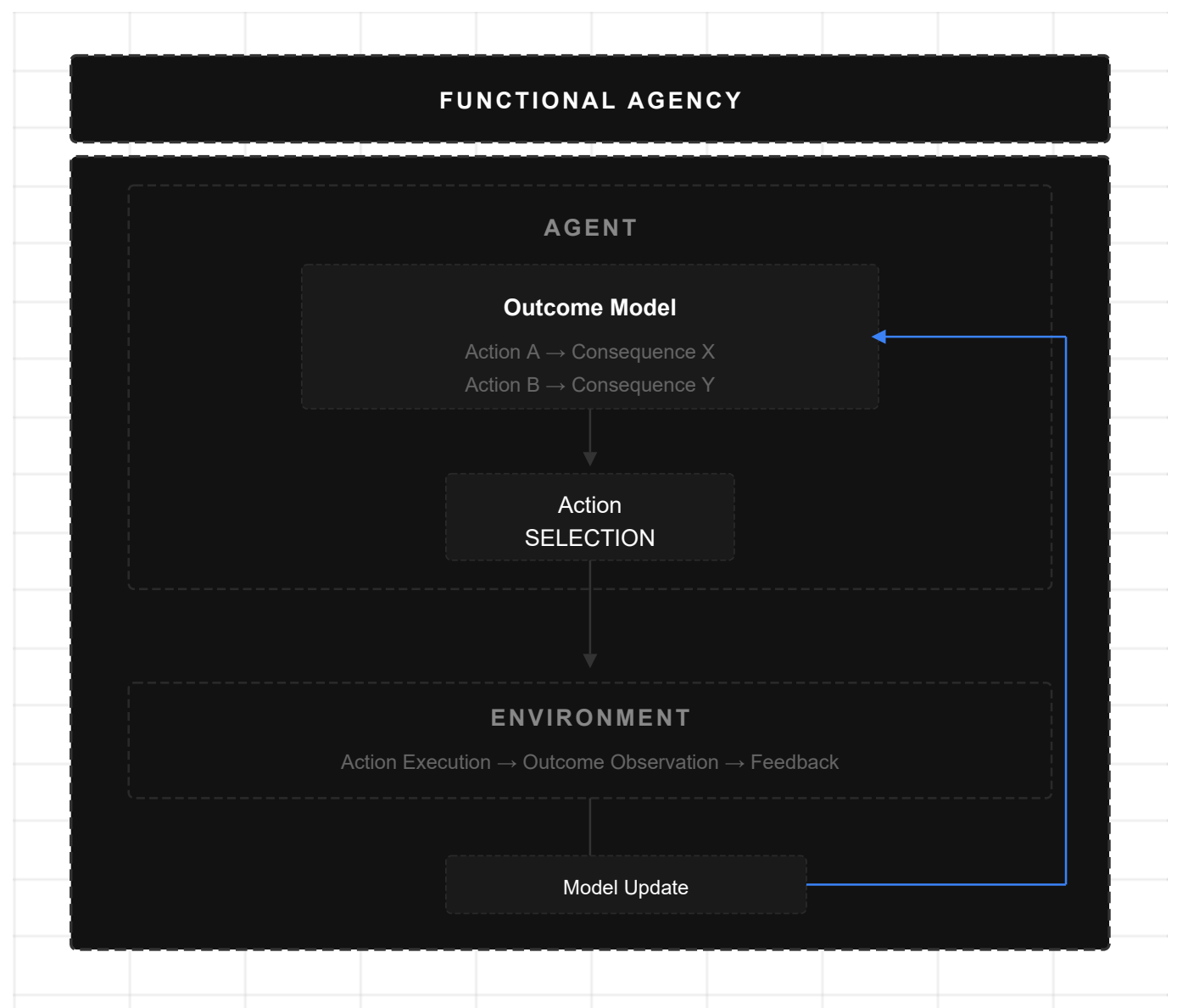
Figure 2: Functional Agency
