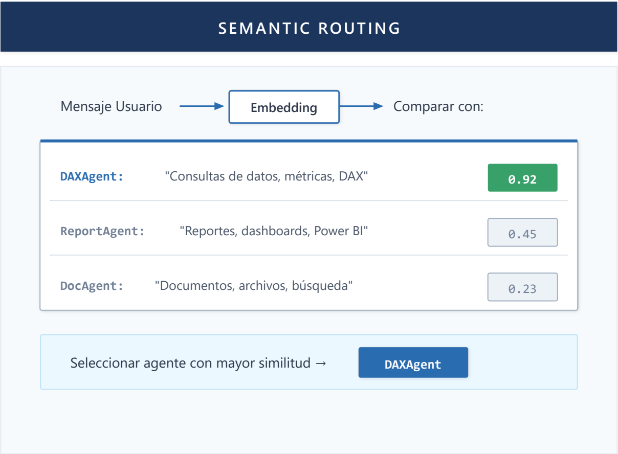
Figura 20: Semantic Routing
