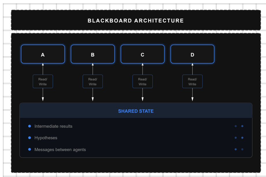
Figure 13: Blackboard Architecture
