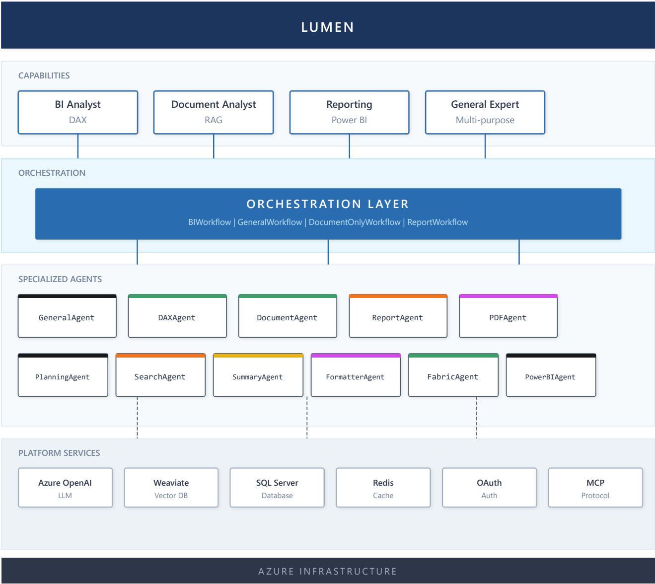
Figure 18: LUMEN Architecture
