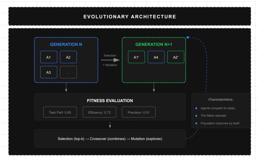
Figure 10: Evolutionary Architecture
