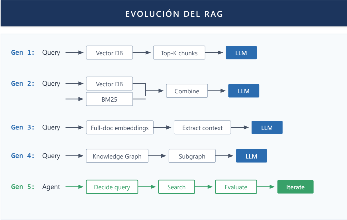
Figure 22: RAG Evolution
