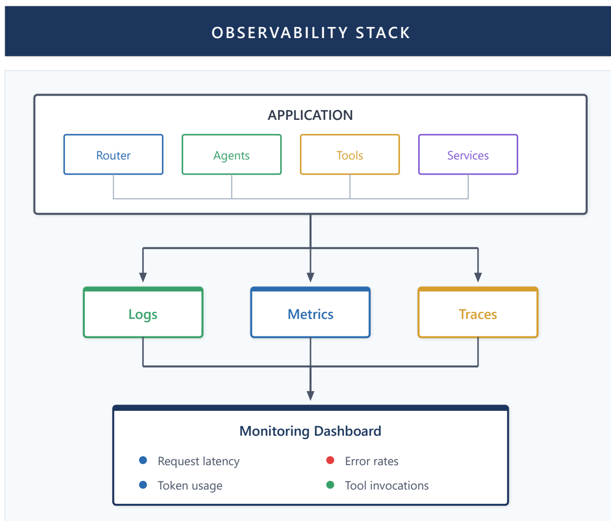
Figura 36: Observability Stack
