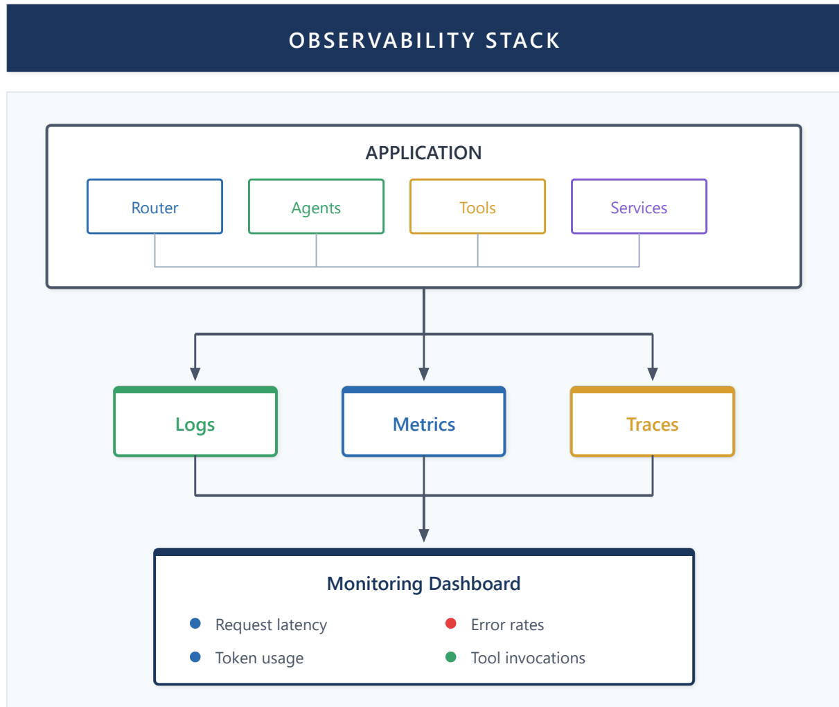
Figure 36: Observability Stack
