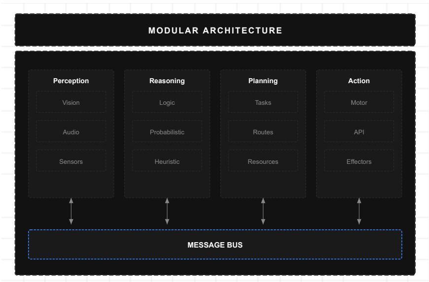
Figure 9: Modular Architecture
