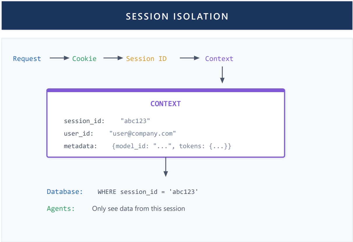
Figure 32: Session Isolation
