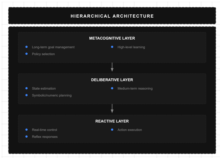
Figure 6: Hierarchical Architecture
