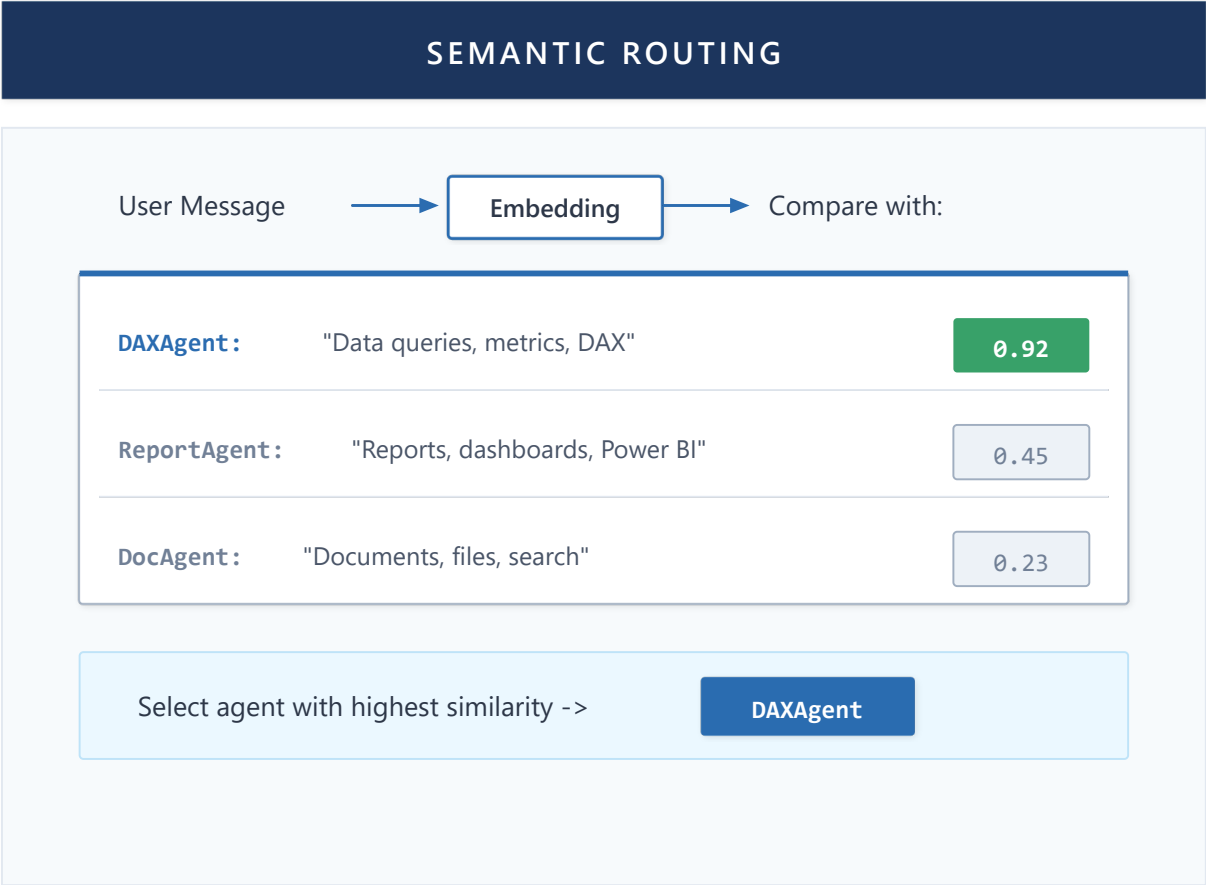
Figure 20: Semantic Routing
