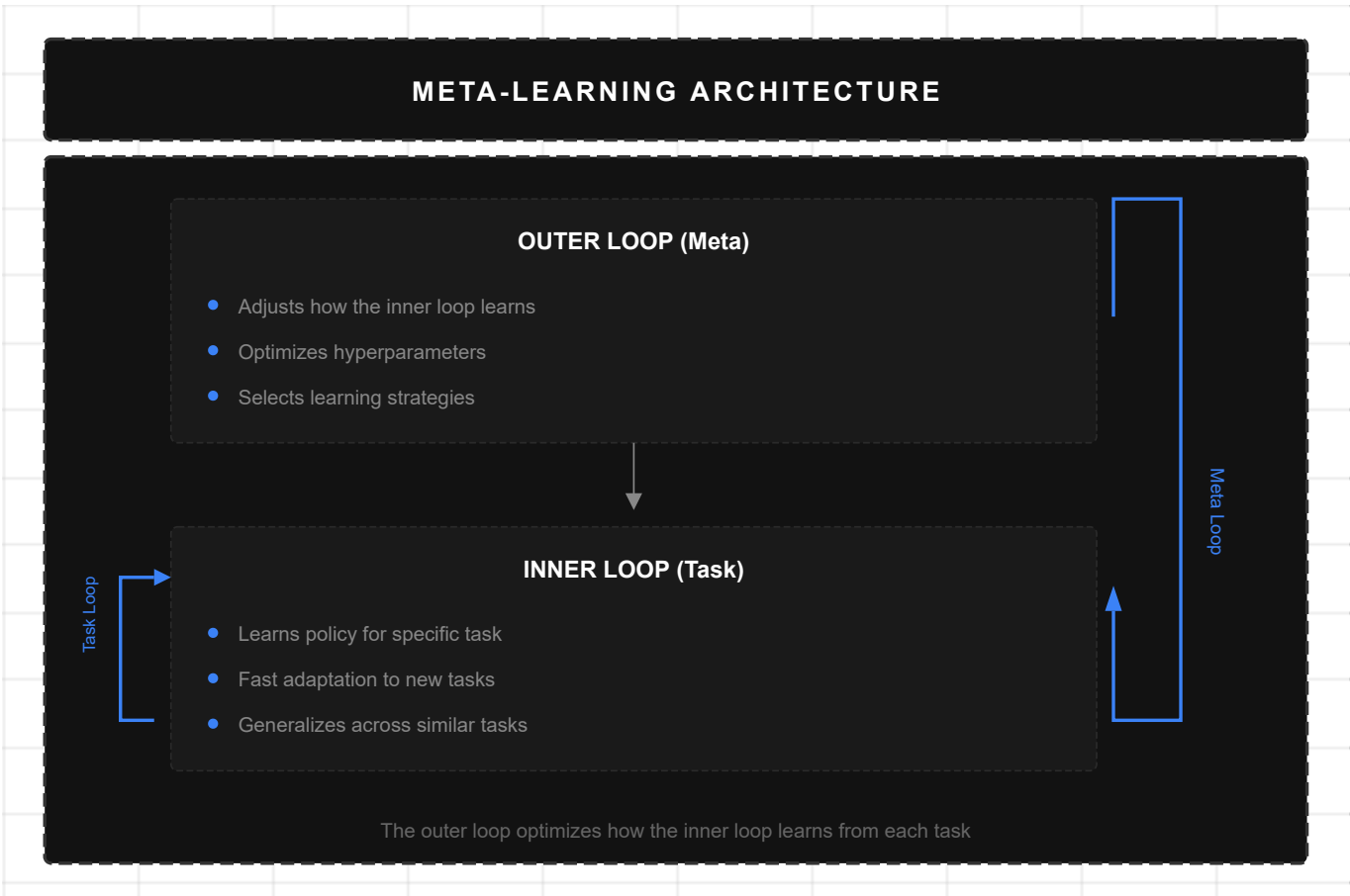
Figure 8: Meta-Learning
