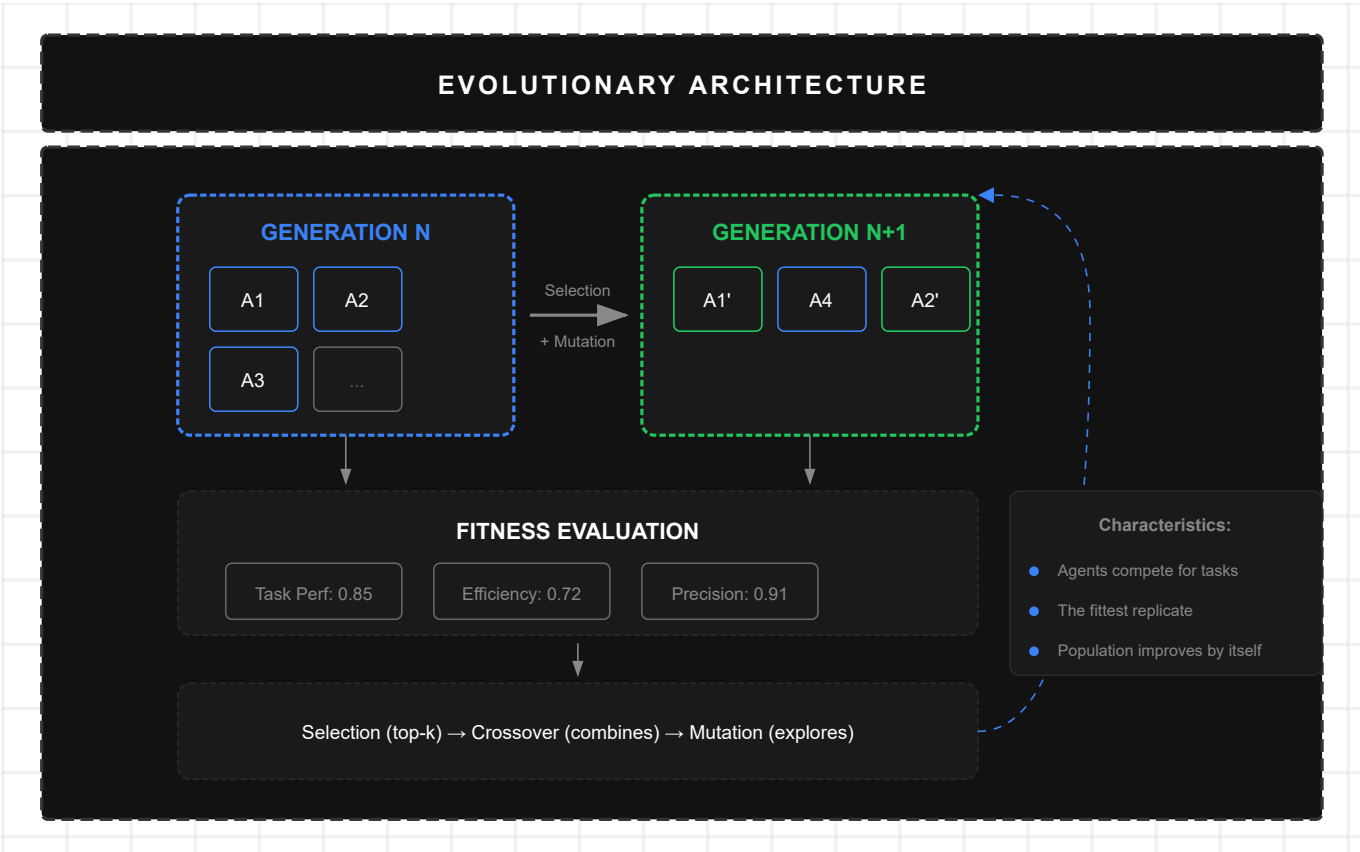
Figure 10: Evolutionary Architecture
