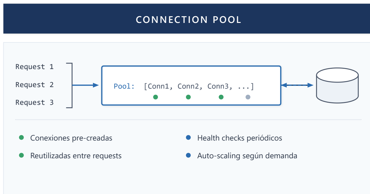
Figure 33: Connection Pool
