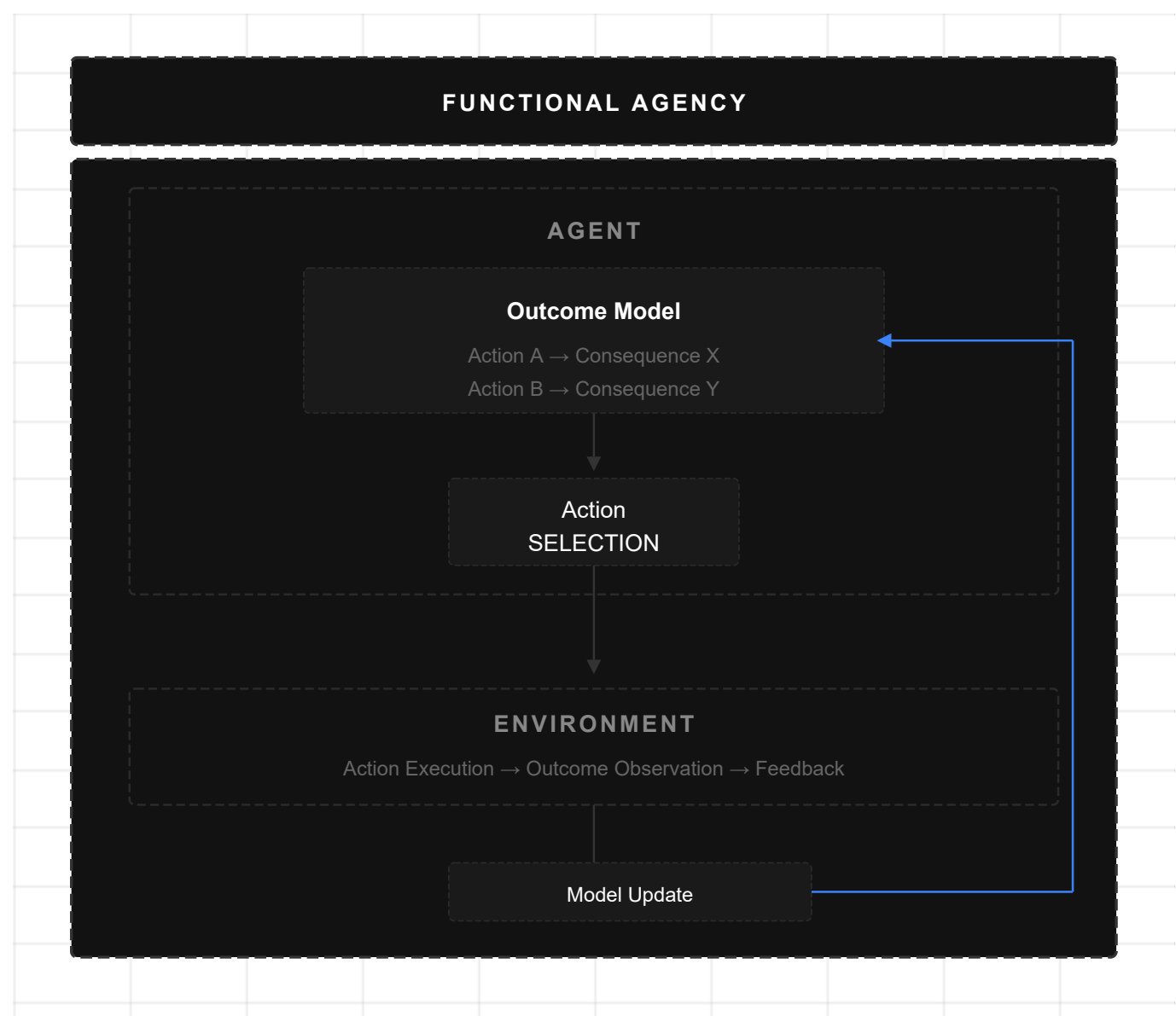
Figure 2: Functional Agency
