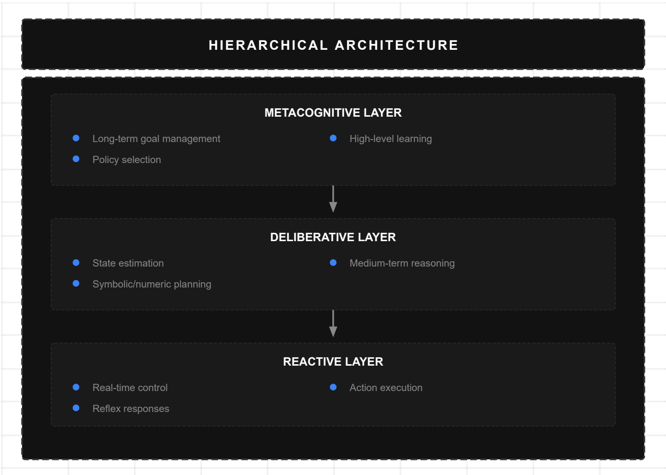
Figure 6: Hierarchical Architecture
