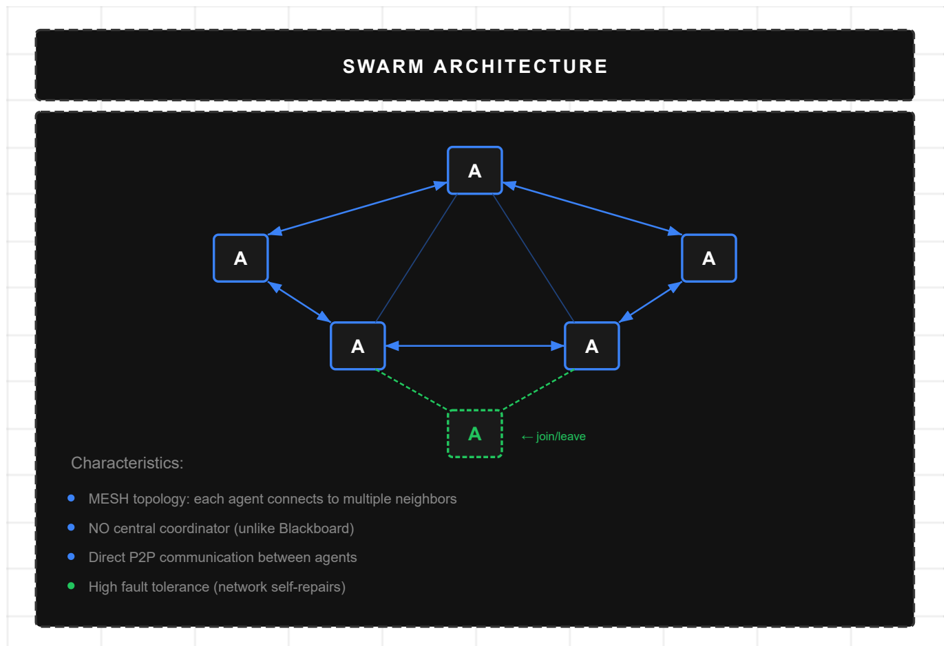
Figure 7: Swarm Architecture
