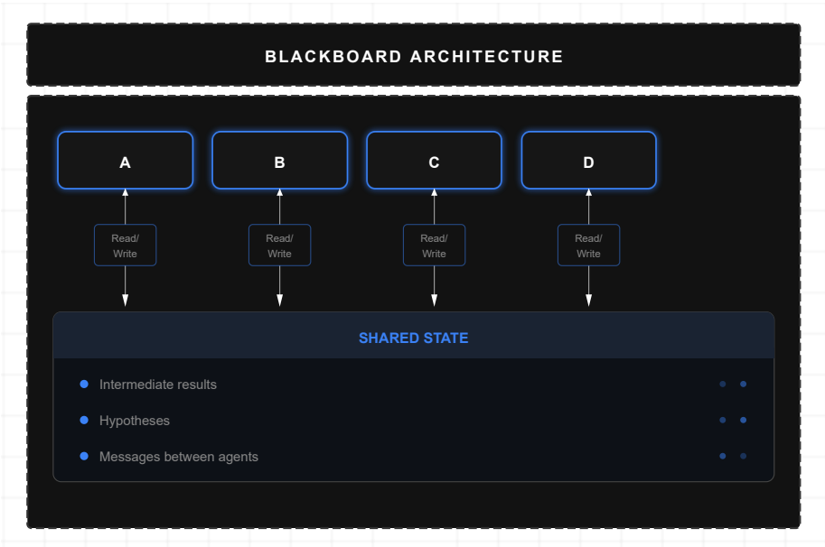
Figure 13: Blackboard Architecture
