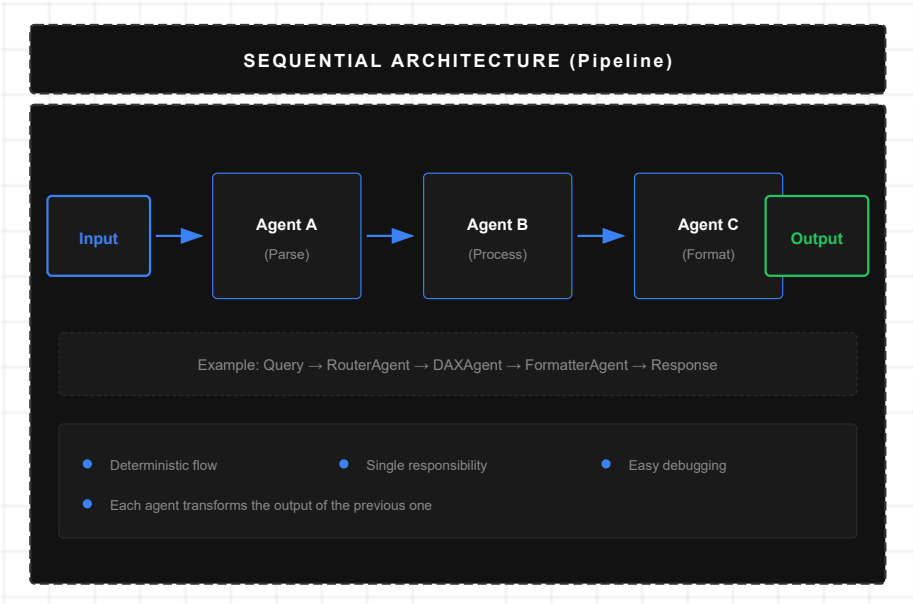
Figure 14: Sequential Architecture
