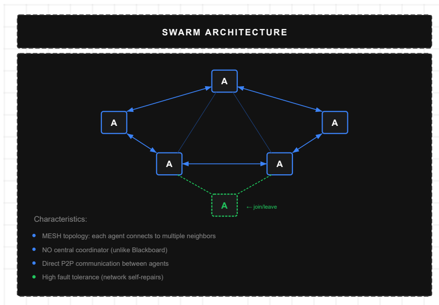
Figure 7: Swarm Architecture
