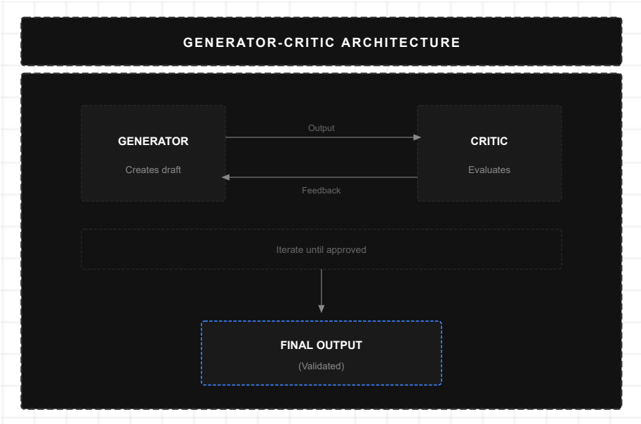
Figure 12: Generator-Critic Architecture
