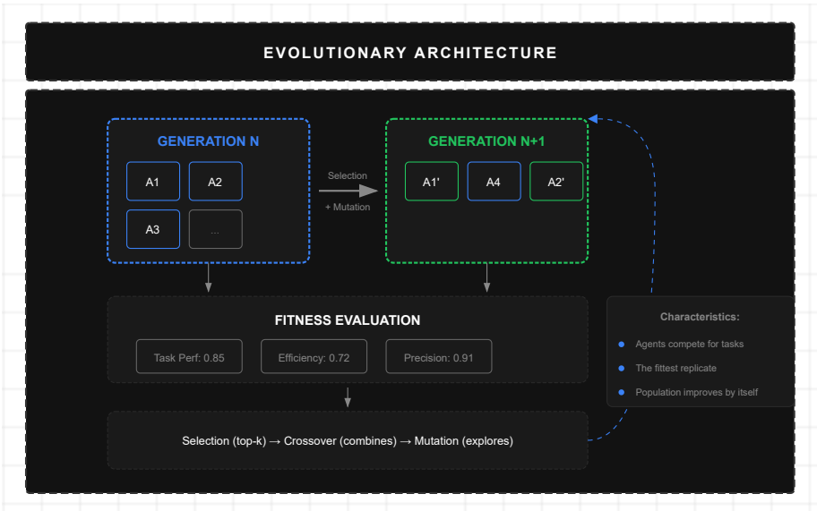
Figure 10: Evolutionary Architecture
