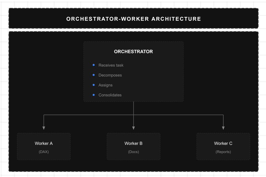
Figure 11: Orchestrator-Worker Architecture
