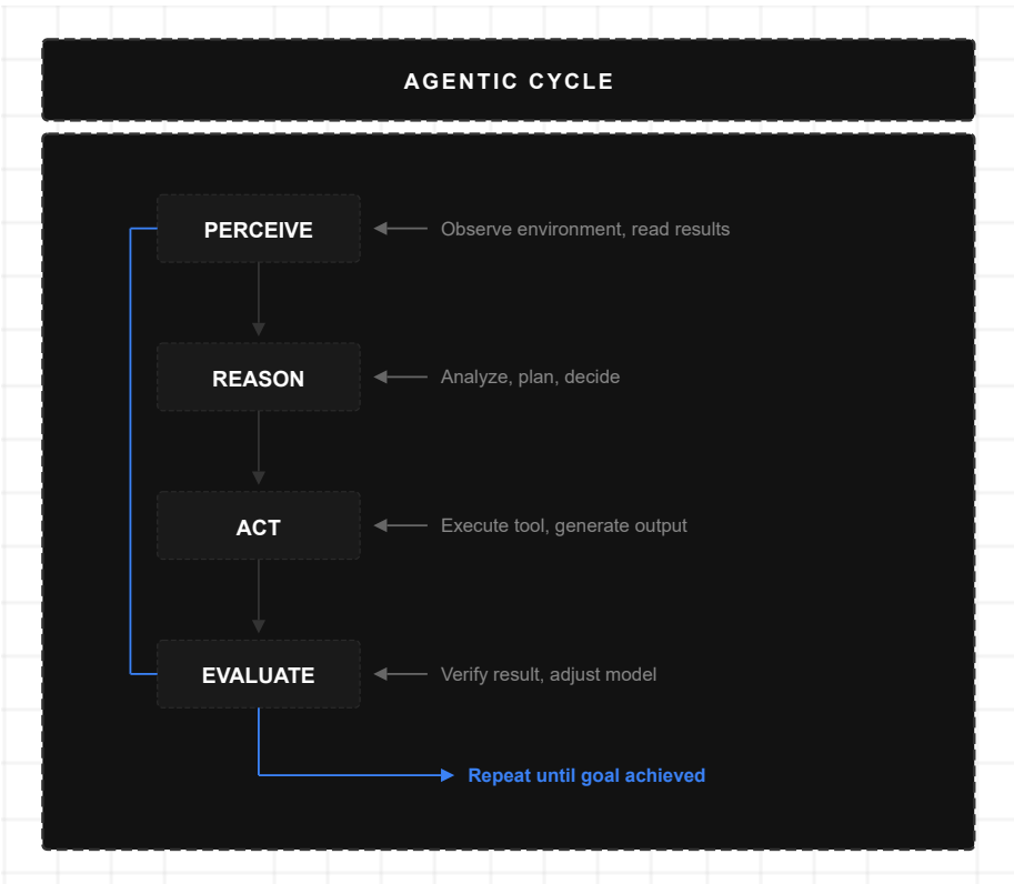
Figure 3: Agentic Cycle
