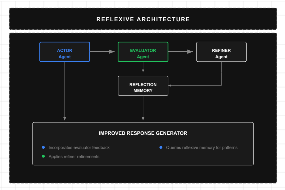
Figure 16: Reflexive Architecture
