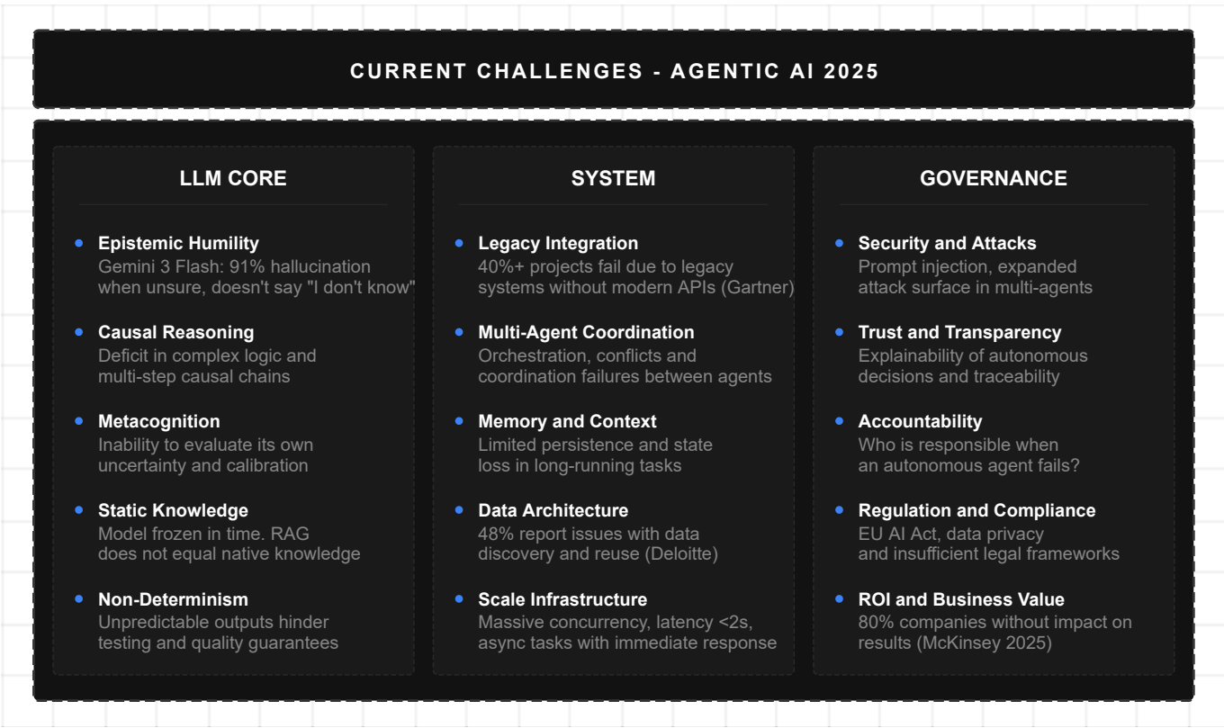
Figure 4: Current Challenges
