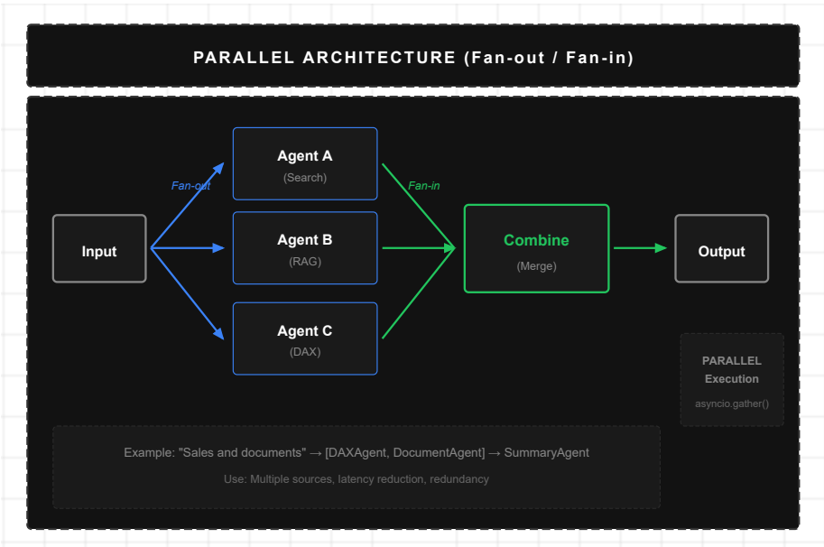
Figure 15: Parallel Architecture
