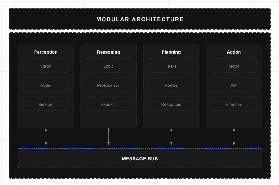
Figure 9: Modular Architecture
