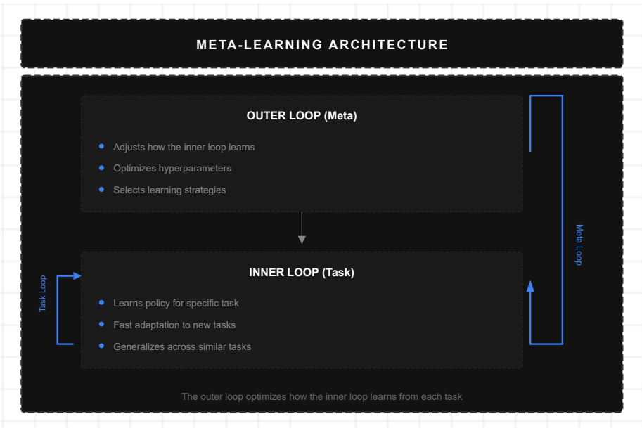
Figure 8: Meta-Learning
