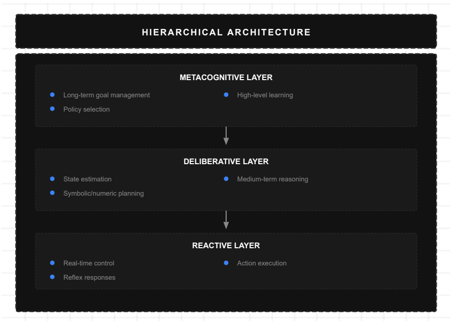
Figure 6: Hierarchical Architecture
