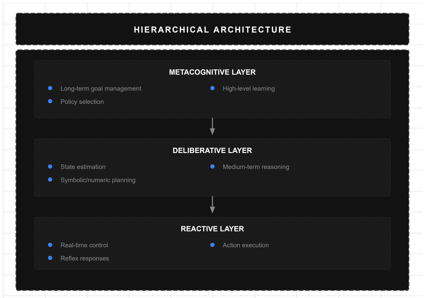
Figure 6: Hierarchical Architecture
