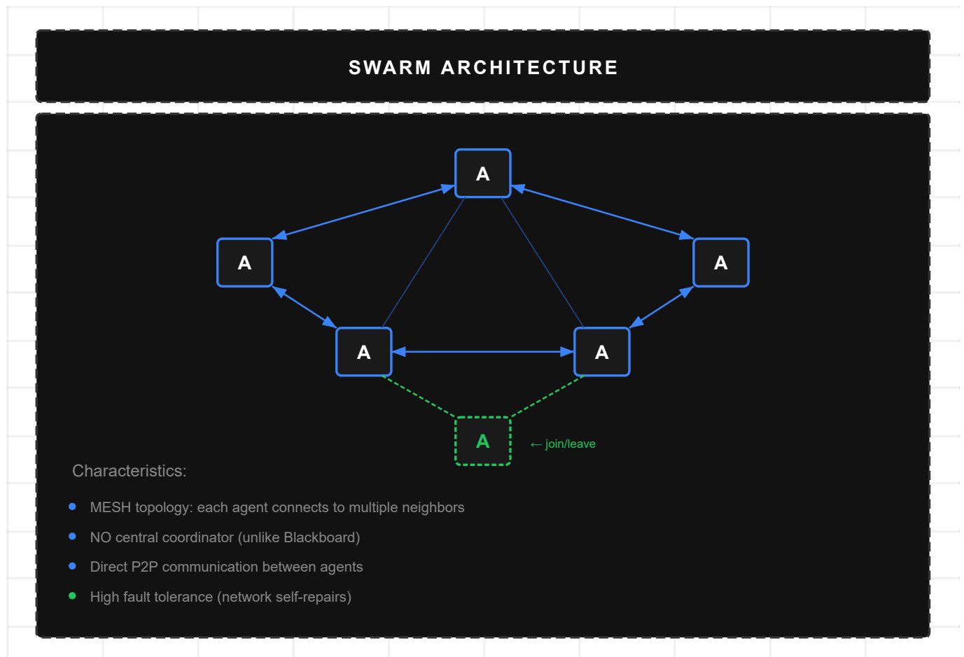
Figure 7: Swarm Architecture
