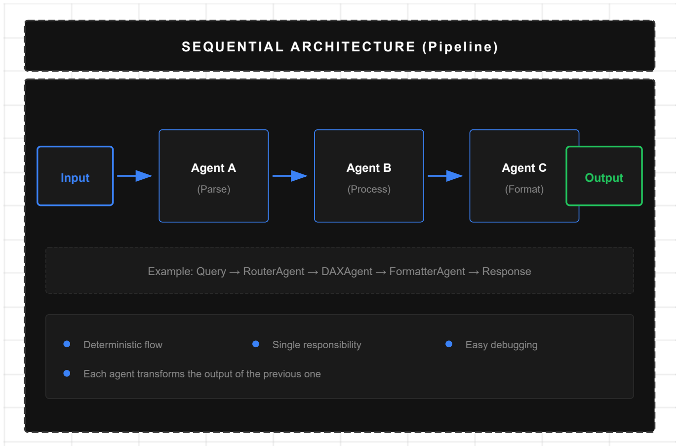
Figure 14: Sequential Architecture
