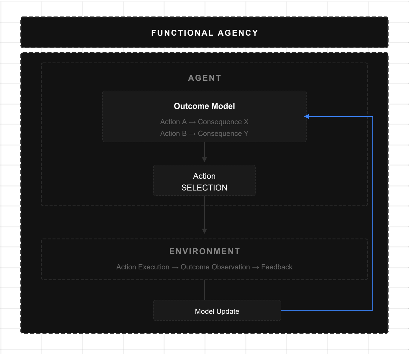
Figure 2: Functional Agency
