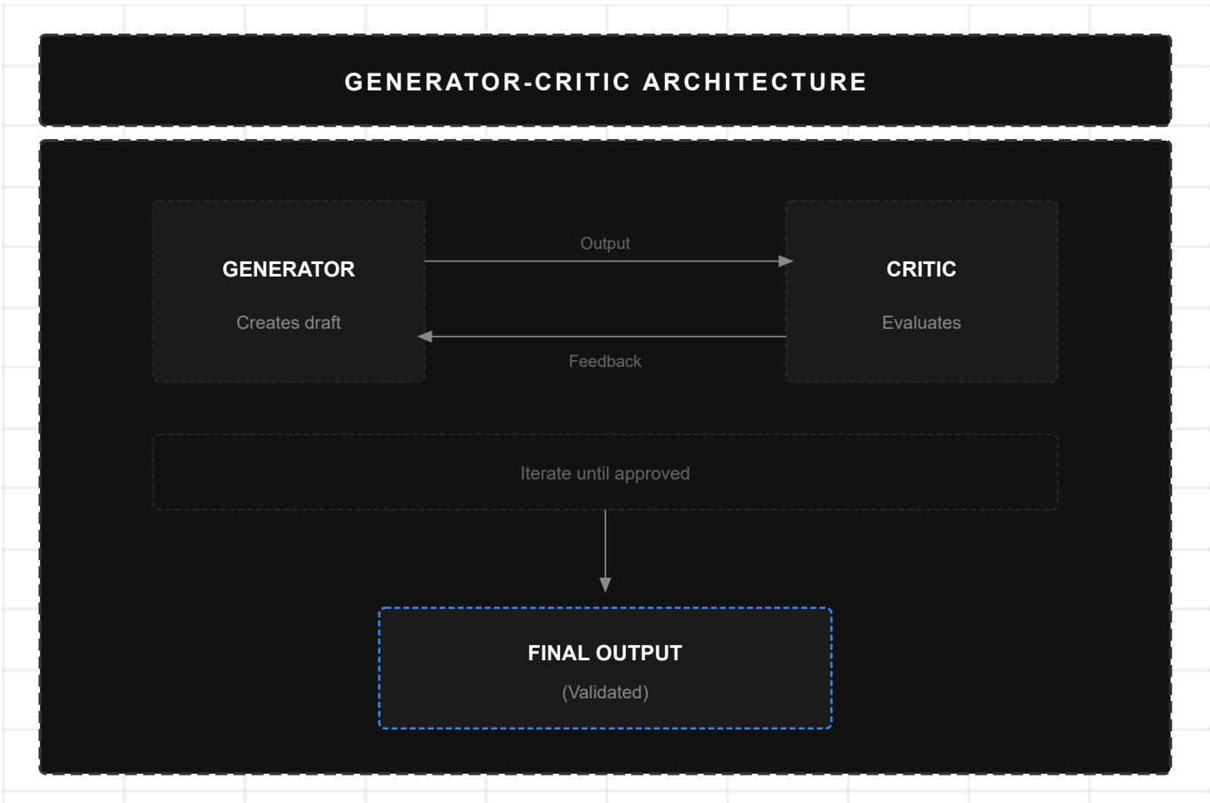
Figure 12: Generator-Critic Architecture
