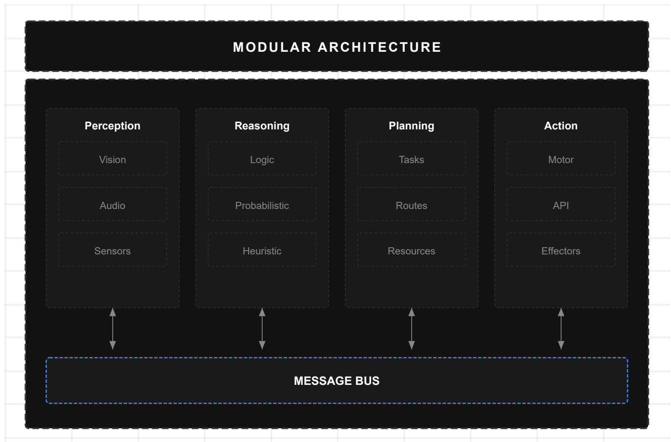
Figure 9: Modular Architecture
