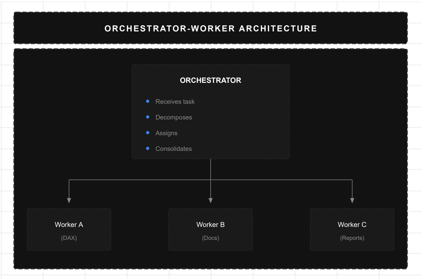
Figure 11: Orchestrator-Worker Architecture
