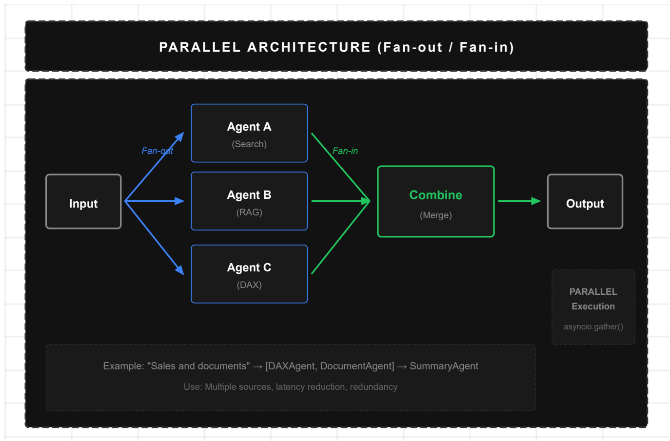
Figure 15: Parallel Architecture
