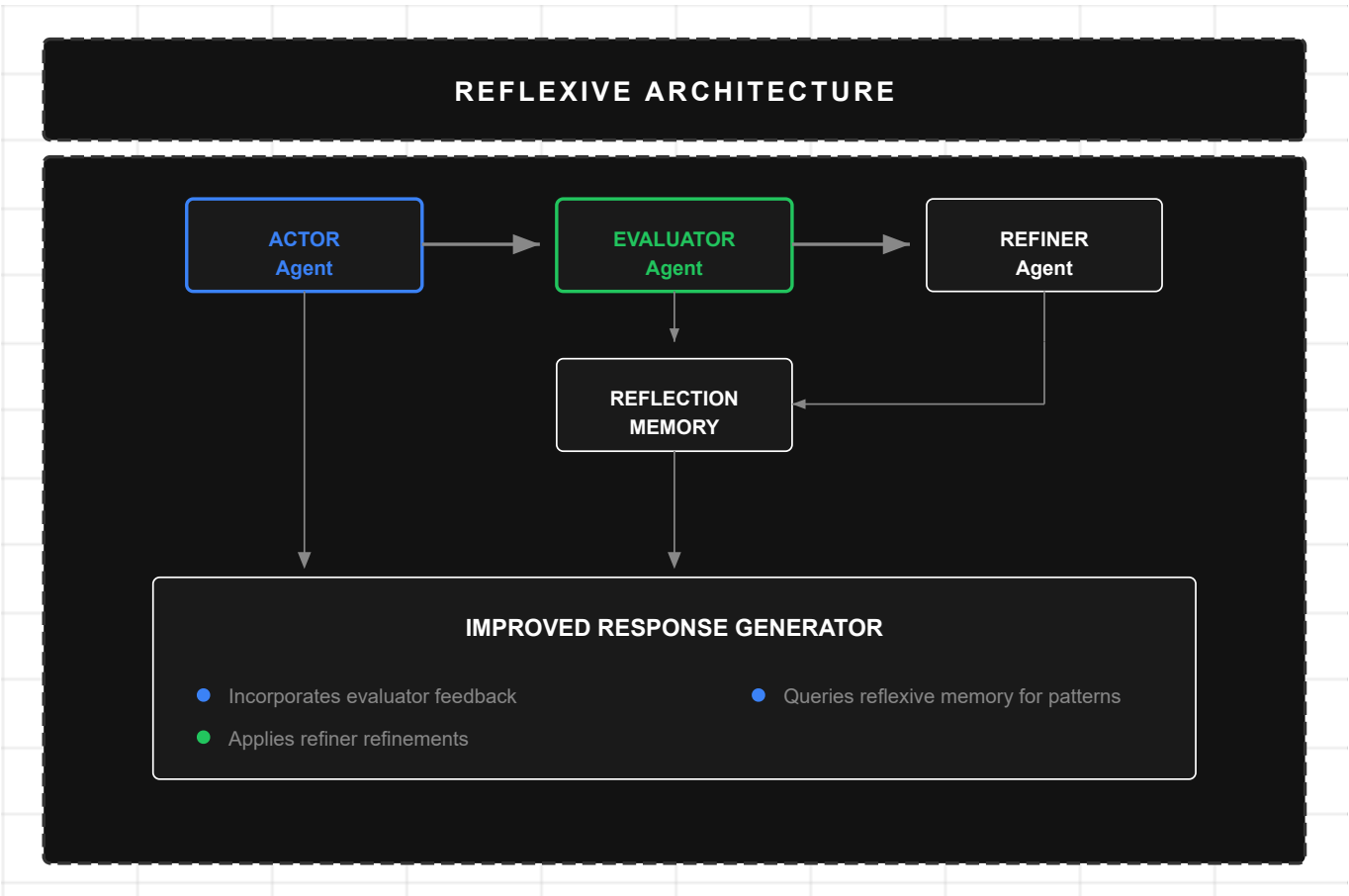
Figure 16: Reflexive Architecture
