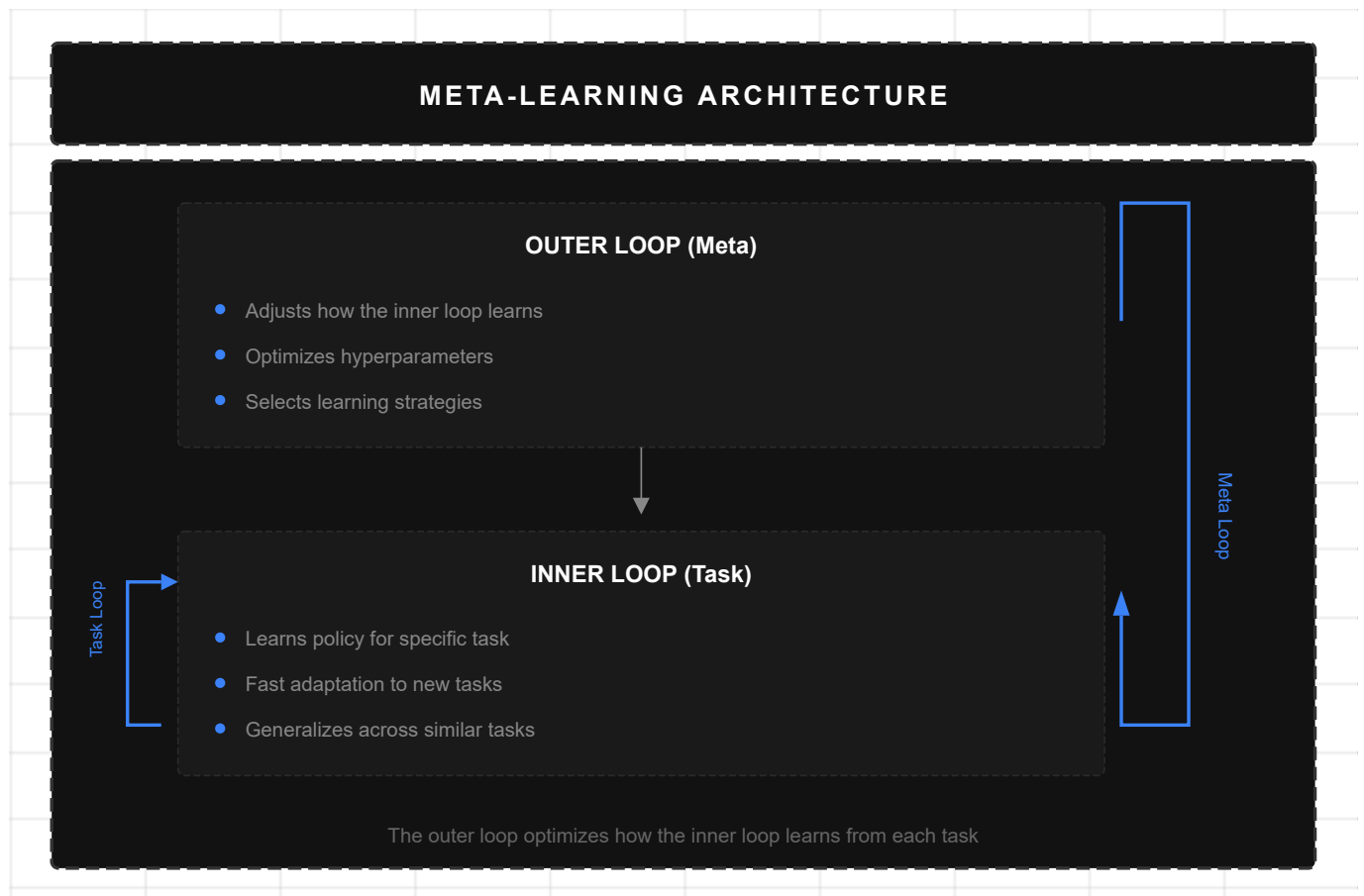
Figure 8: Meta-Learning
