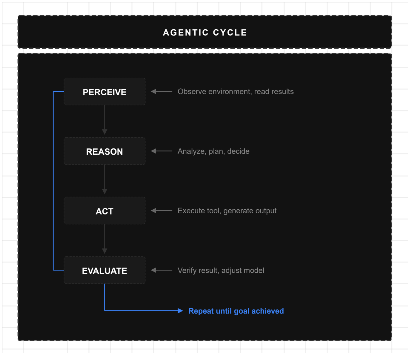
Figure 3: Agentic Cycle
