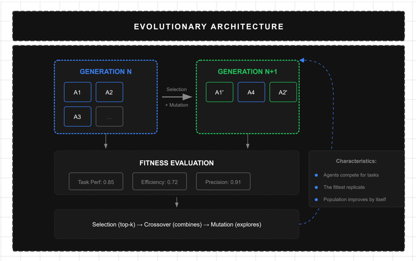
Figure 10: Evolutionary Architecture
