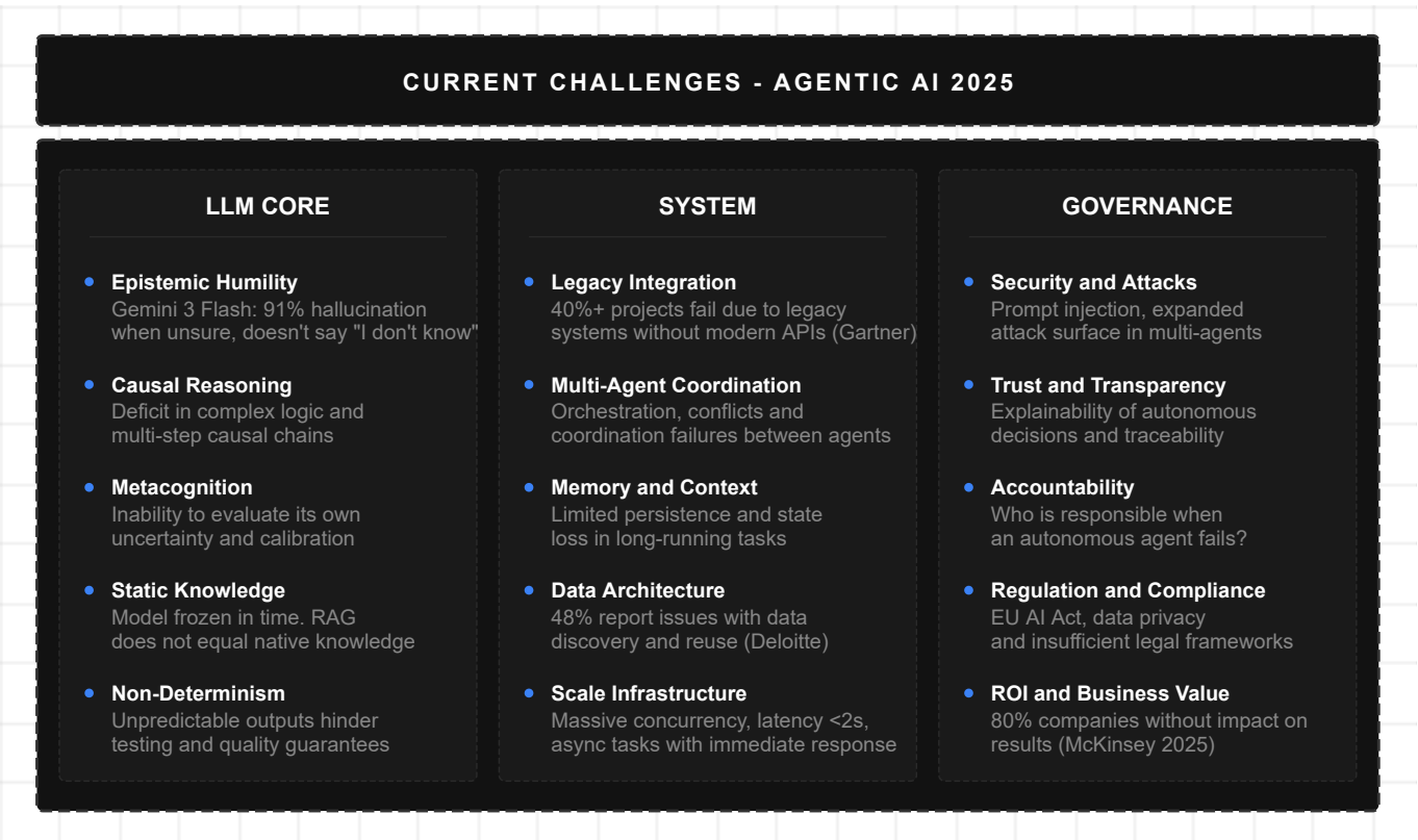
Figure 4: Current Challenges
