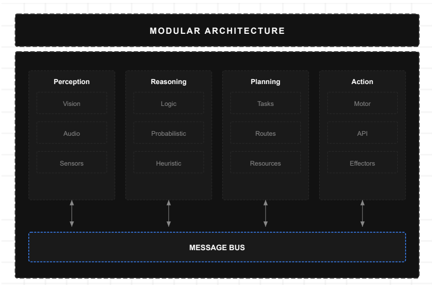
Figure 9: Modular Architecture
