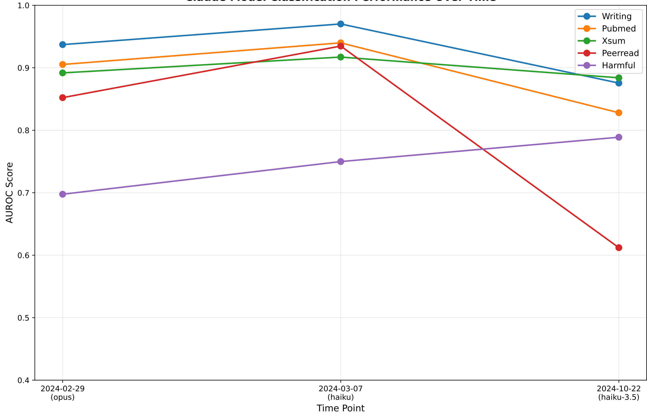
Claude Model Classification Performance Over Time
