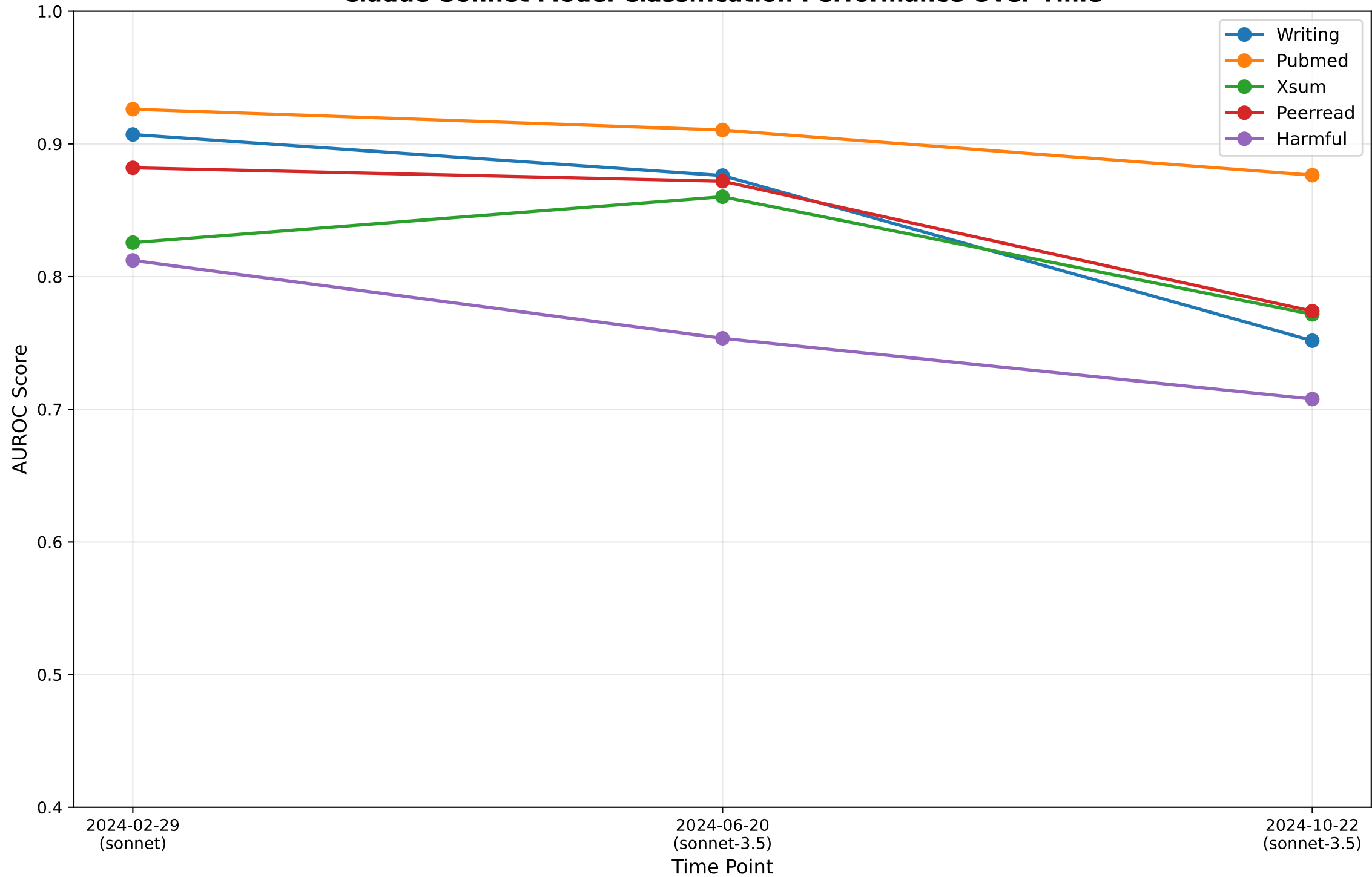
Claude-Sonnet Model Classification Performance Over Time
