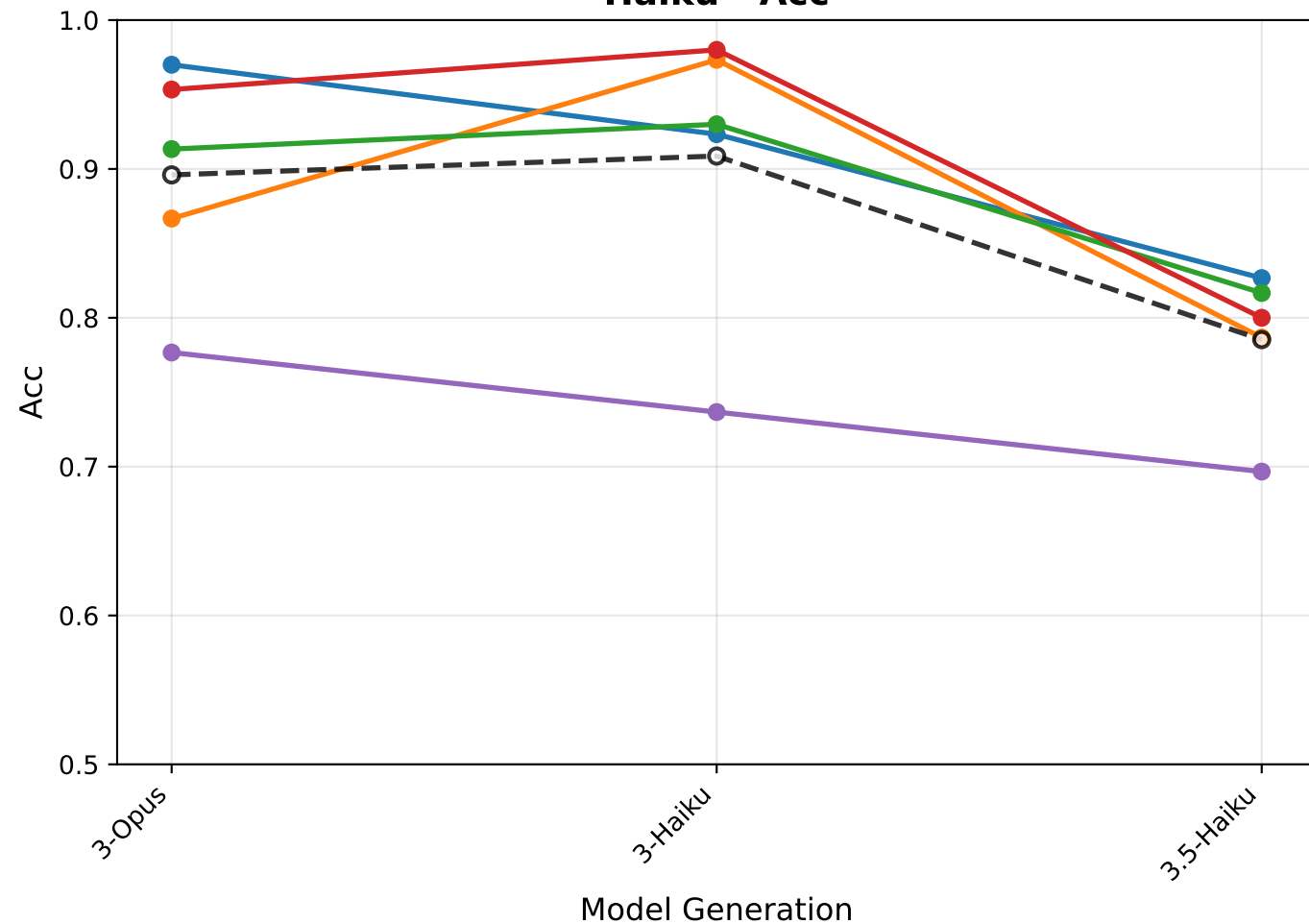
Haiku - Acc
