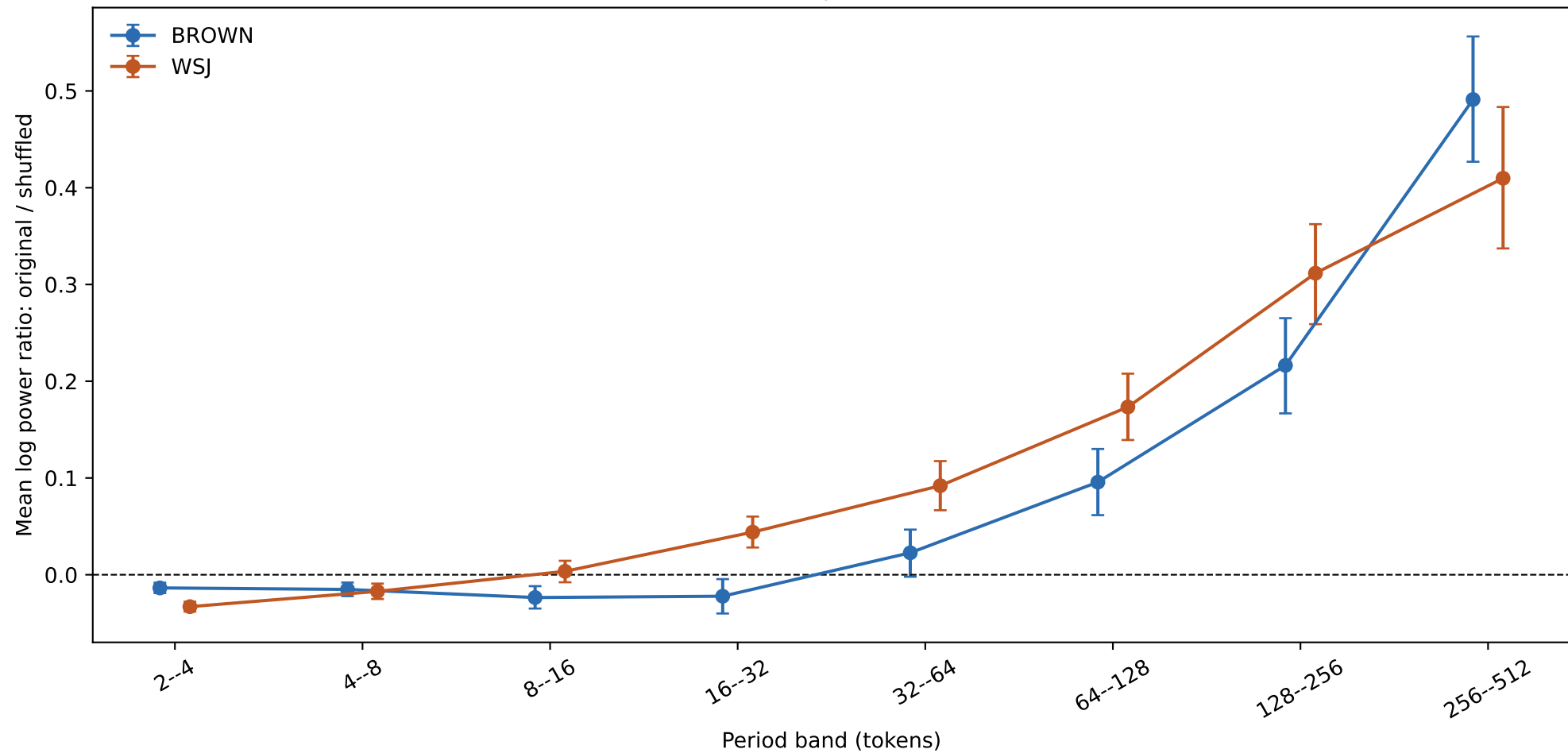
Document-level spectrum validation
