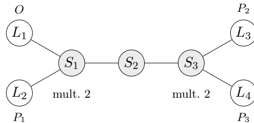
FIGURE 1. The affine- D_6 dual graph of an I_2^* fiber of X_{\mathrm{III}} , marked at the representative fiber T = 0 : legs L_1, \dots, L_4 have multiplicity 1, spine components S_1, S_2, S_3 have multiplicity 2. The zero section O and the three nonzero 2-torsion sections P_1, P_2, P_3 occupy the four legs individually (Lemma 5.6), forcing (Lemma 5.7) every component – legs and spine alike – to be individually Galois-fixed.
