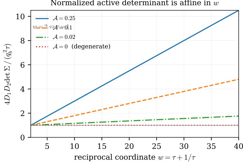
Figure 2: The normalized determinant (18) as a function of the reciprocal coordinate w , for several values of the slope. The dependence is exactly affine, with value 1 at w = 2 (the homogeneous point \tau = 1 ). In the rank-one case the slope is \mathcal{A} = c^2 s^2 \nu^2 \in [0, 1/4) ; in general it is K/q_b^2 , nonnegative for an admissible family (Definition 19).
