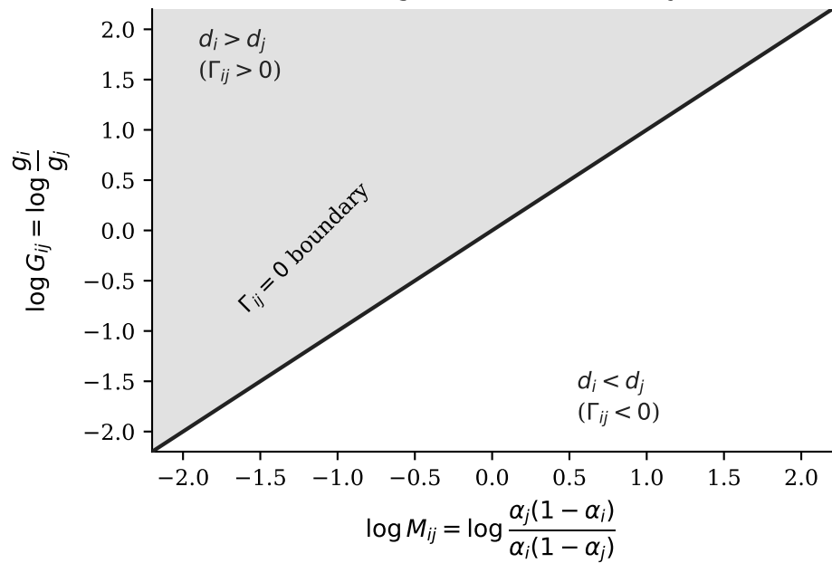
(b) Pairwise ranking-inversion boundary (Thm.~5.1)
