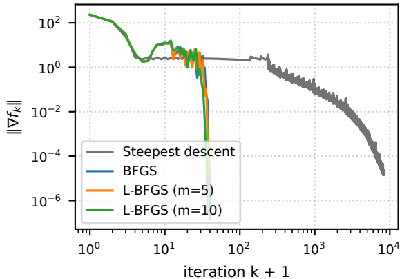
Rosenbrock, n = 2
