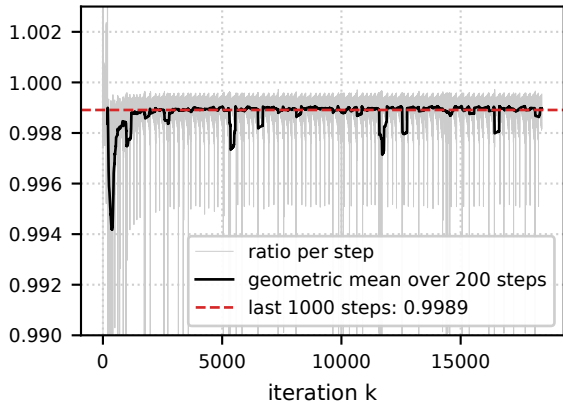
Steepest descent: ratio stays near 1
