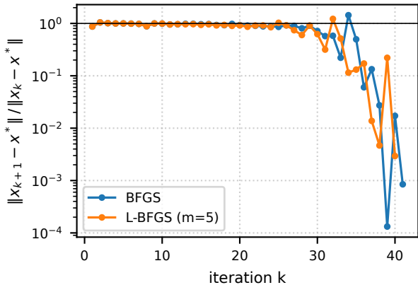
Quasi-Newton: ratios tend to 0
