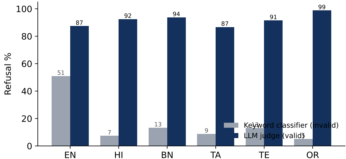
Measuring refusal: keyword scoring hides 70–90 pp of Indic refusals (sarvam-m)
