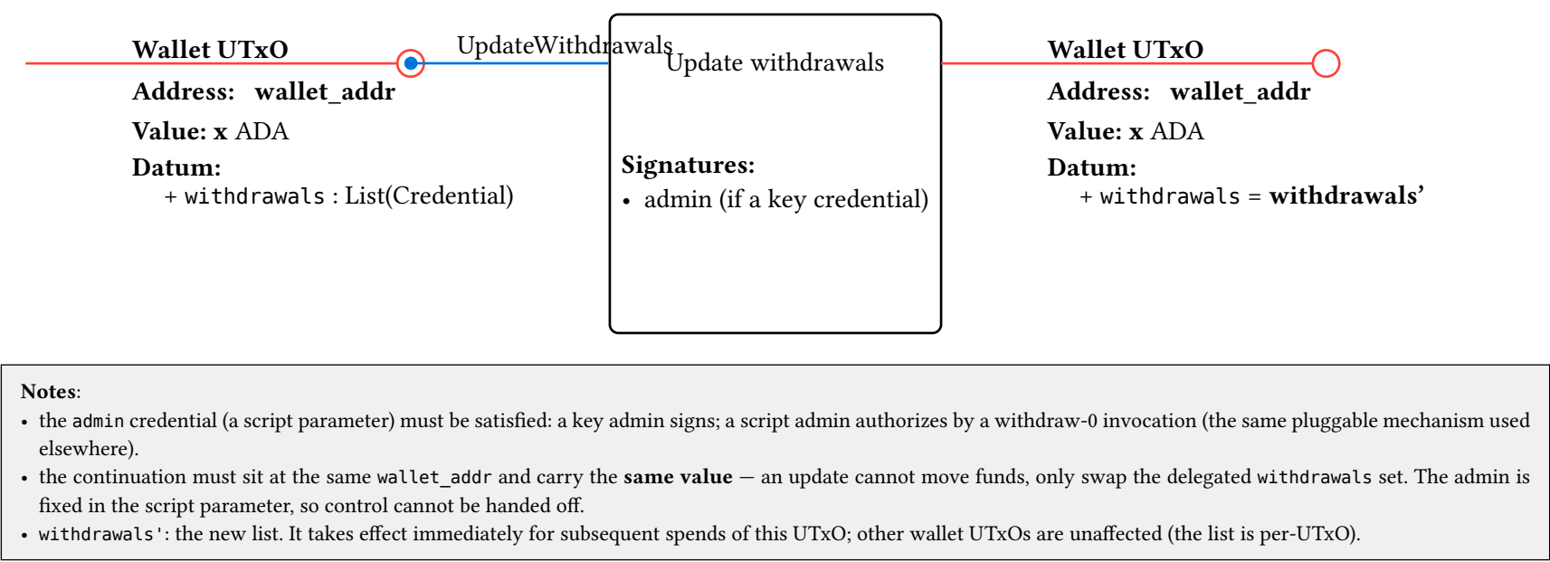
Figure 2: Update withdrawals (per-UTxO)
