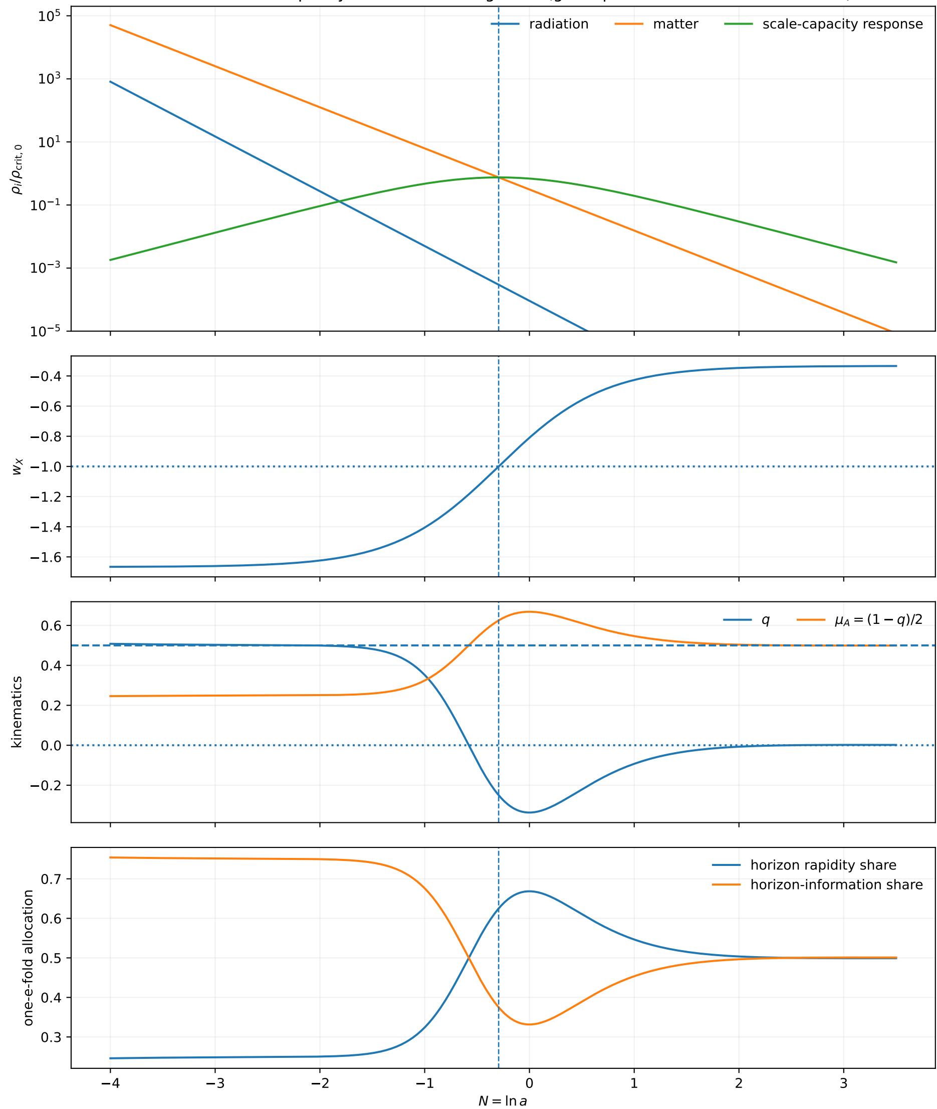
Parameter-free capacity-normalized background (given present matter/radiation state)
