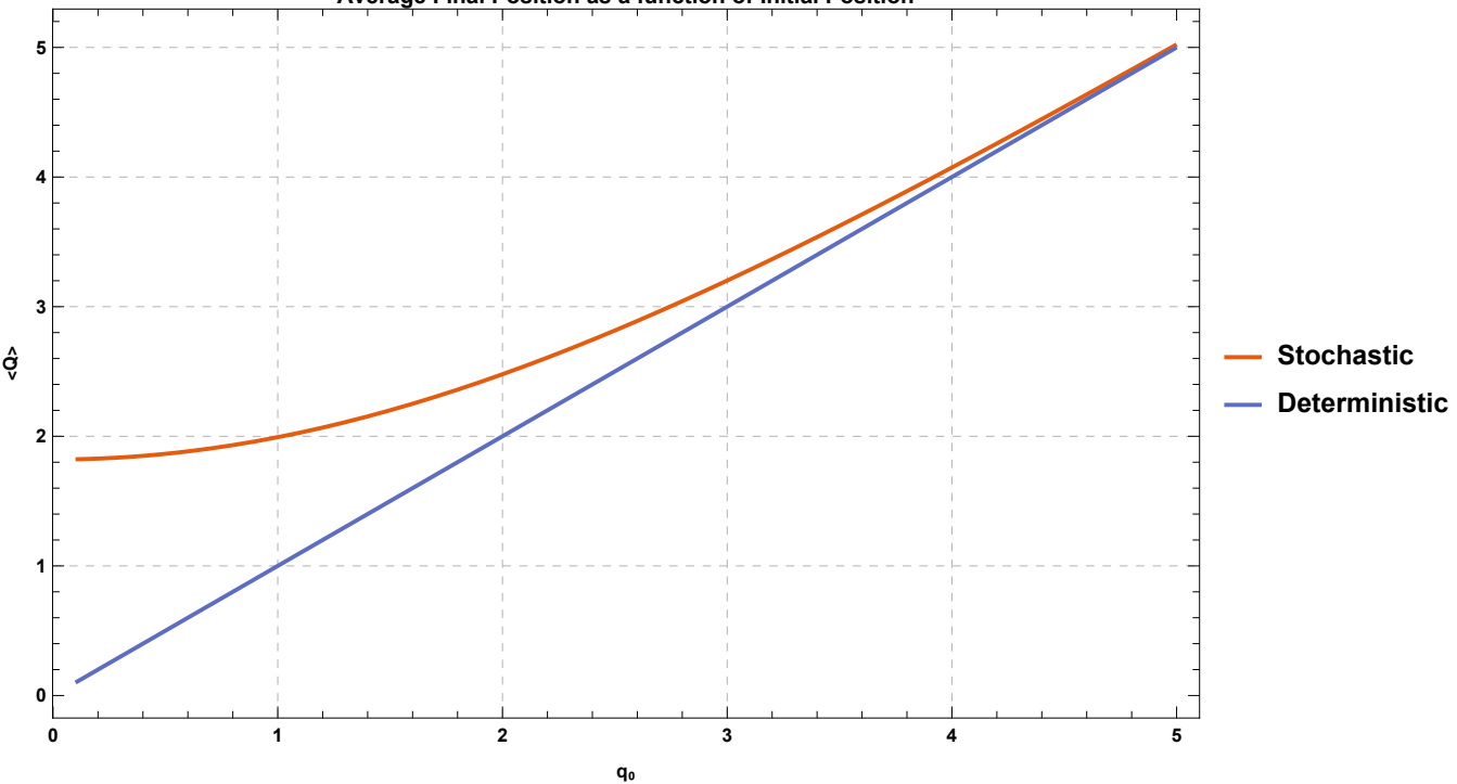
Average Final Position as a function of Initial Position
