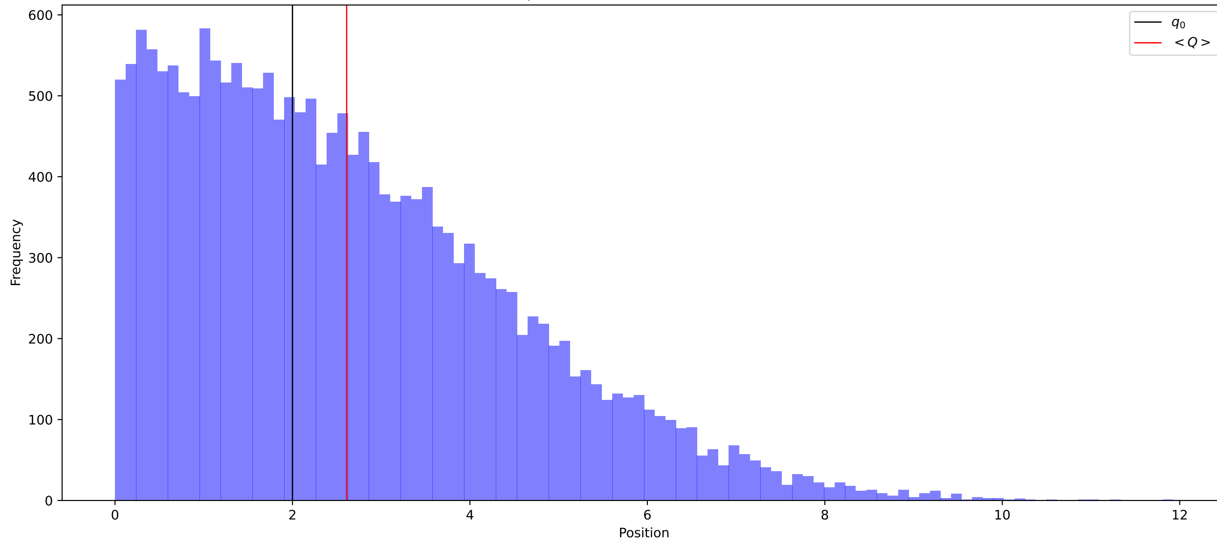
Final distribution of positions Q after 5.00 seconds with reflective wall
