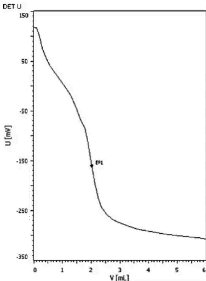
FIG. 2 Illustrative Titration Curve of Biodiesel Sample
