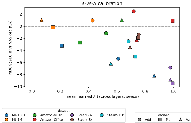
Figure 2: \lambda -vs- \Delta calibration: each marker is one (dataset, variant) cell. x -axis = mean learned \lambda across attention layers and seeds (Table 4); y -axis = mean test-NDCG@10 relative \Delta vs SASRec. Top-right would be the predicted “model uses intensity and gains”; observed: empty. Bottom-right is “model uses intensity and loses”, where Steam clusters.
