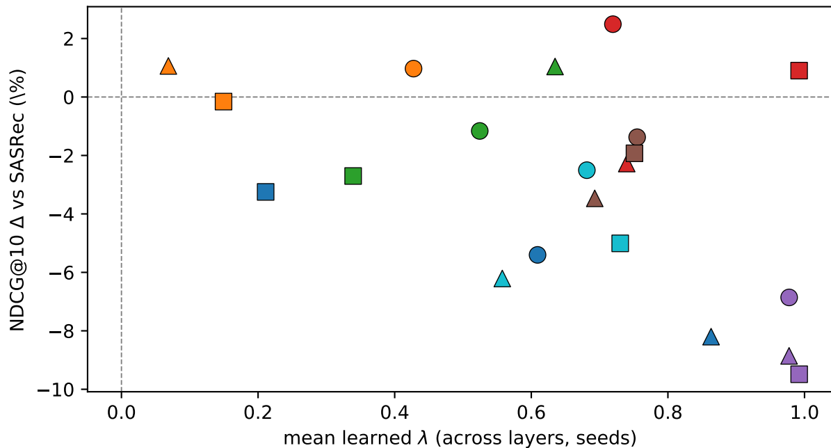
\lambda -vs- \Delta calibration
