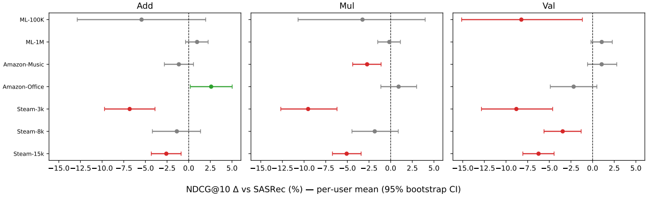
Figure 1: Per-user paired bootstrap ( B=2000 ) on aligned NDCG@10 differences vs SASRec, pooled across five seeds. Three panels, one per variant; within each panel every row is one dataset and rows share the common \Delta x-axis. Centre = mean per-user \Delta , whiskers = 95% percentile CI. Red markers have CI entirely below zero; green entirely above; grey cross zero. No robust positive cell exists for NDCG@10.
