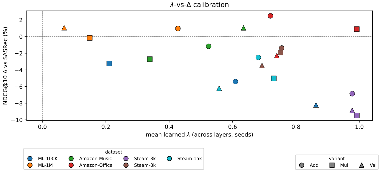
Figure 2: \lambda -vs- \Delta calibration: each marker is one (dataset, variant) cell. x -axis = mean learned \lambda across attention layers and seeds (Table 4); y -axis = mean test-NDCG@10 relative \Delta vs SASRec. Top-right would be the predicted “model uses intensity and gains”; observed: empty. Bottom-right is “model uses intensity and loses”, where Steam clusters.
