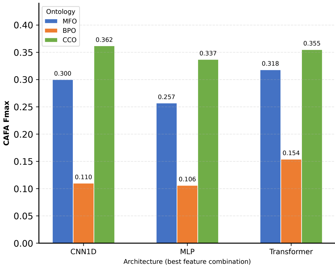
Per-Ontology Fmax — Best Model per Architecture
