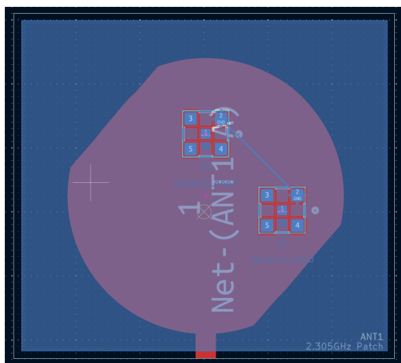
(a) B.Cu view
