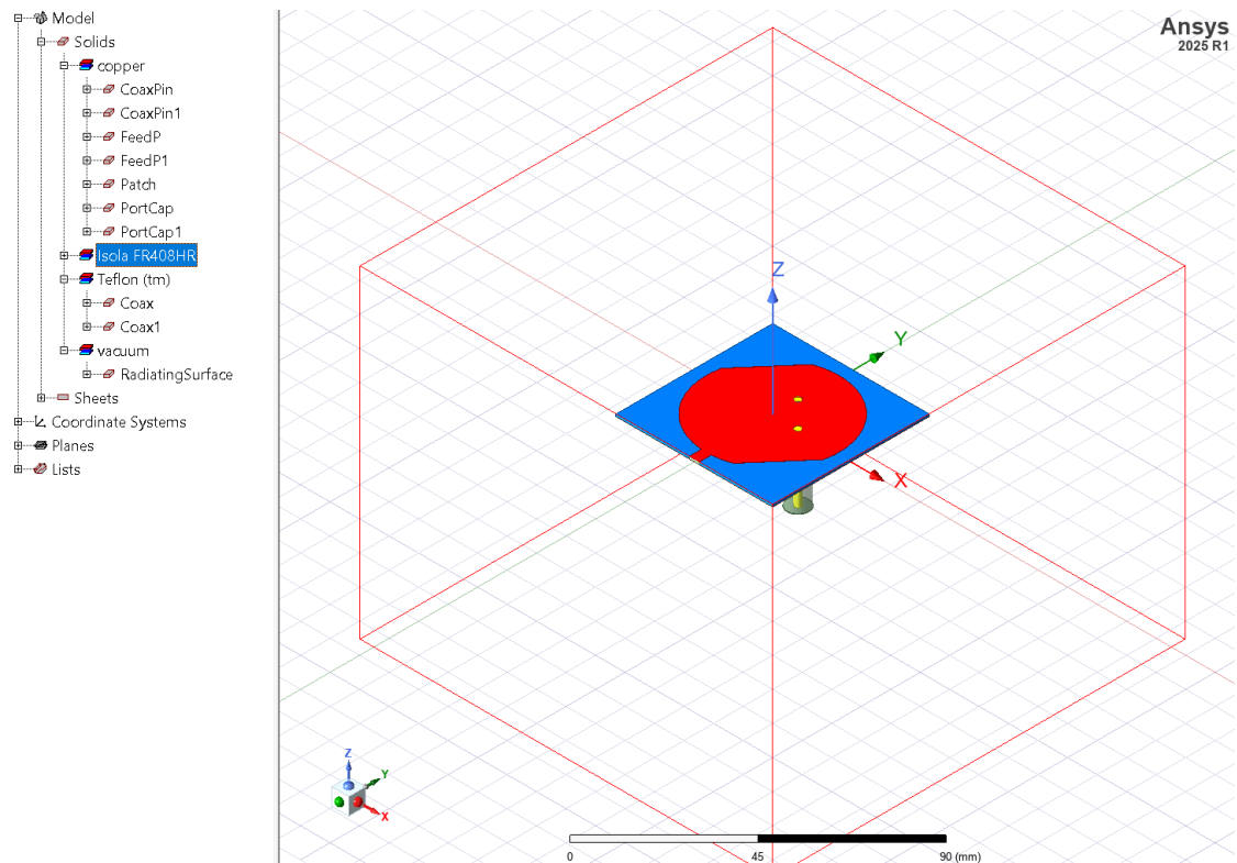
Figure 2.2: HFSS model, final circular patch
