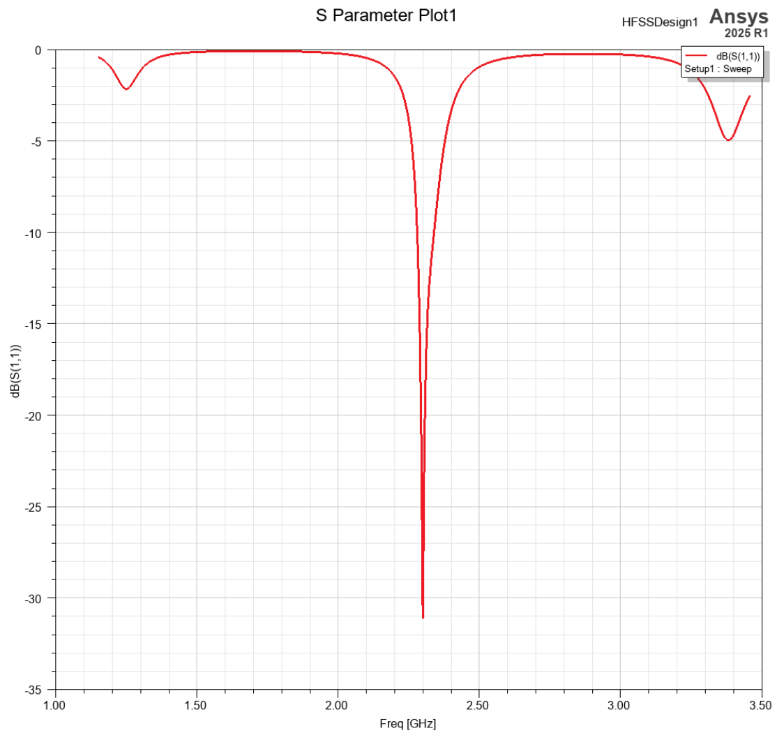
Figure 3.1: S11, final circular patch
