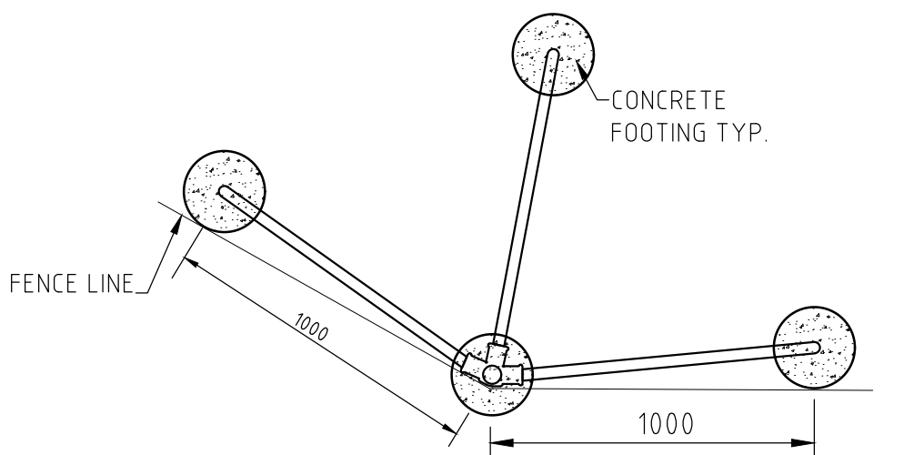
CORNER POST FOOTING PLAN(>90) SCALE 1:20
