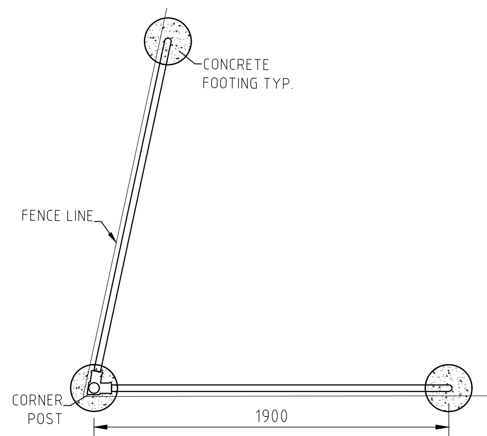
CORNER POST FOOTING PLAN (<90) SCALE 1:20
