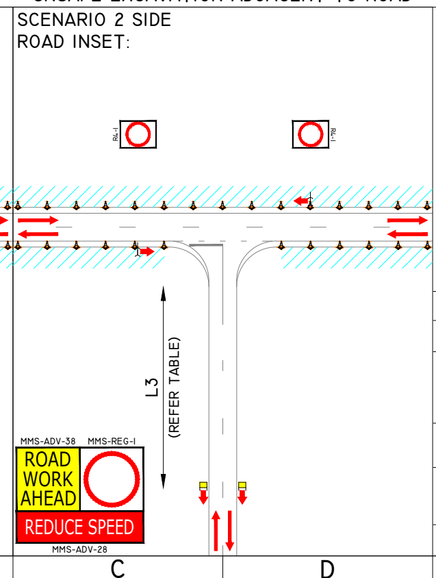
SCENARIO 2 UNSAFE EXCAVATION ADJACENT TO ROAD
