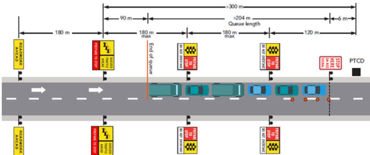
Figure 4.6: Avoiding end of queue collisions (> 300 m)
