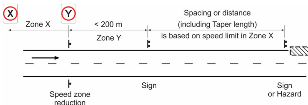
Figure 2.2(a) – Sign or hazard within 200 m of a speed zone change
