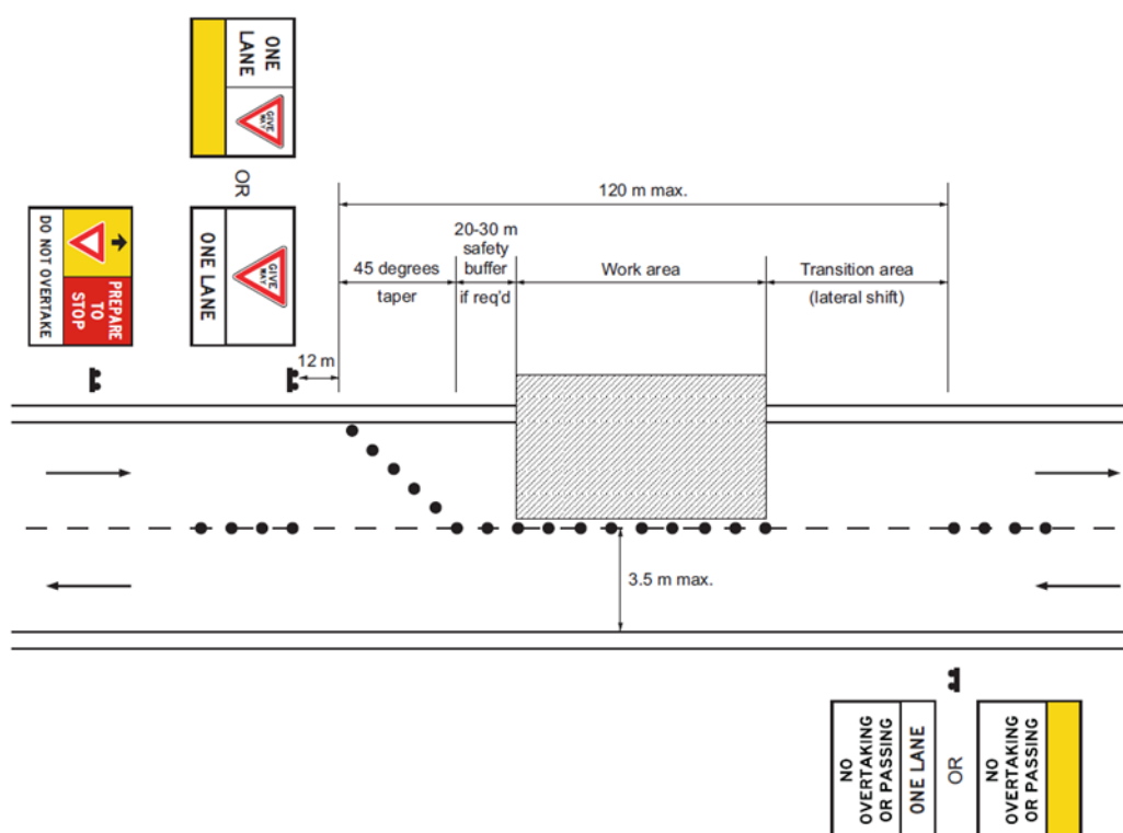
Figure 5.4.4(a) – Example layout using GIVE WAY signs
